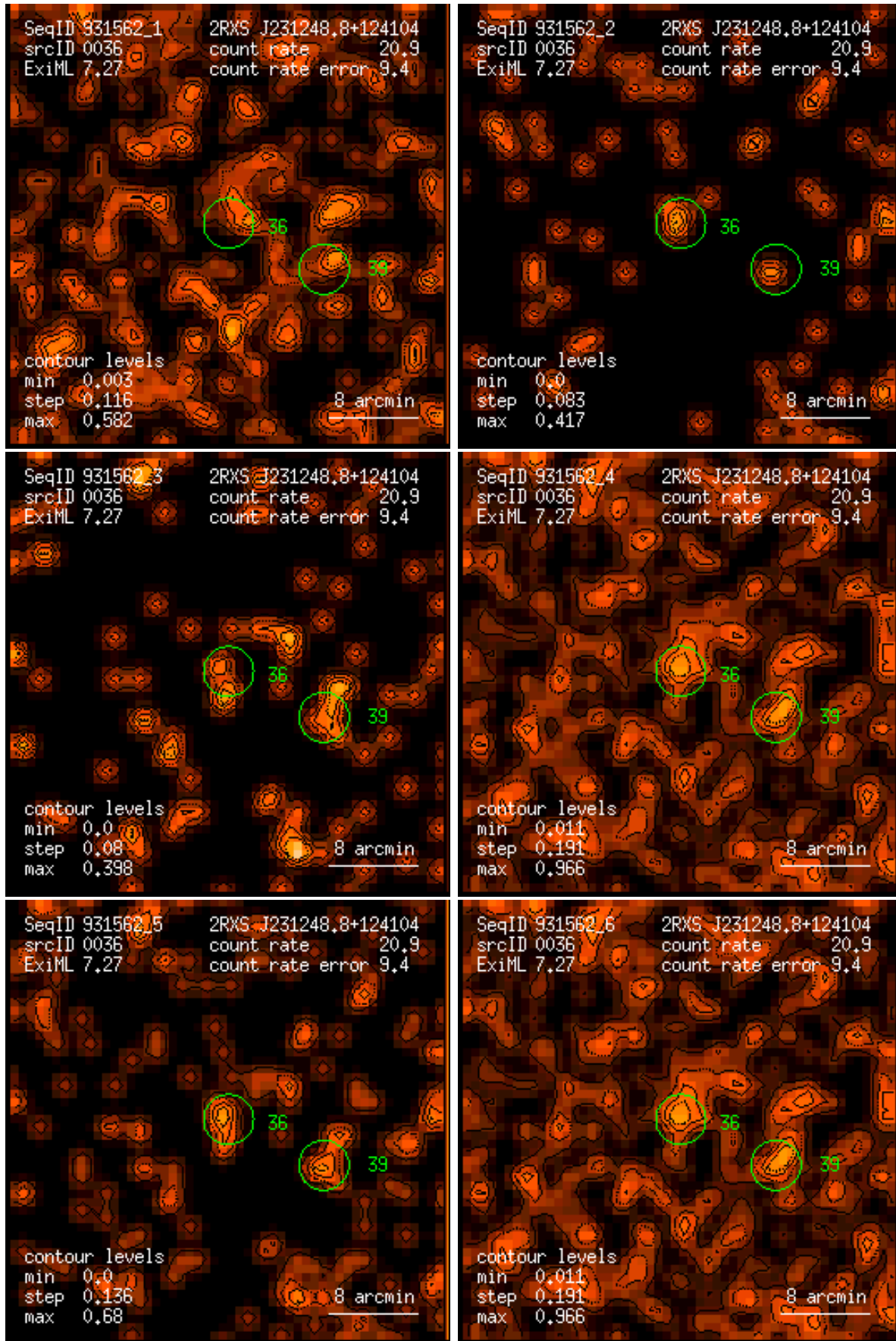
Figure 36: RASS 931562: detection 0036: band rate images, Gaussian filter: (1) PSPC channels 11 – 41, (2) 52 – 90, (3) 91 – 201, (4) 11 – 235, (5) 52 – 201, (6) 11 – 201. Broad band rates in counts/ks. Band rate contour levels in counts/ks/arcmin 2 .
