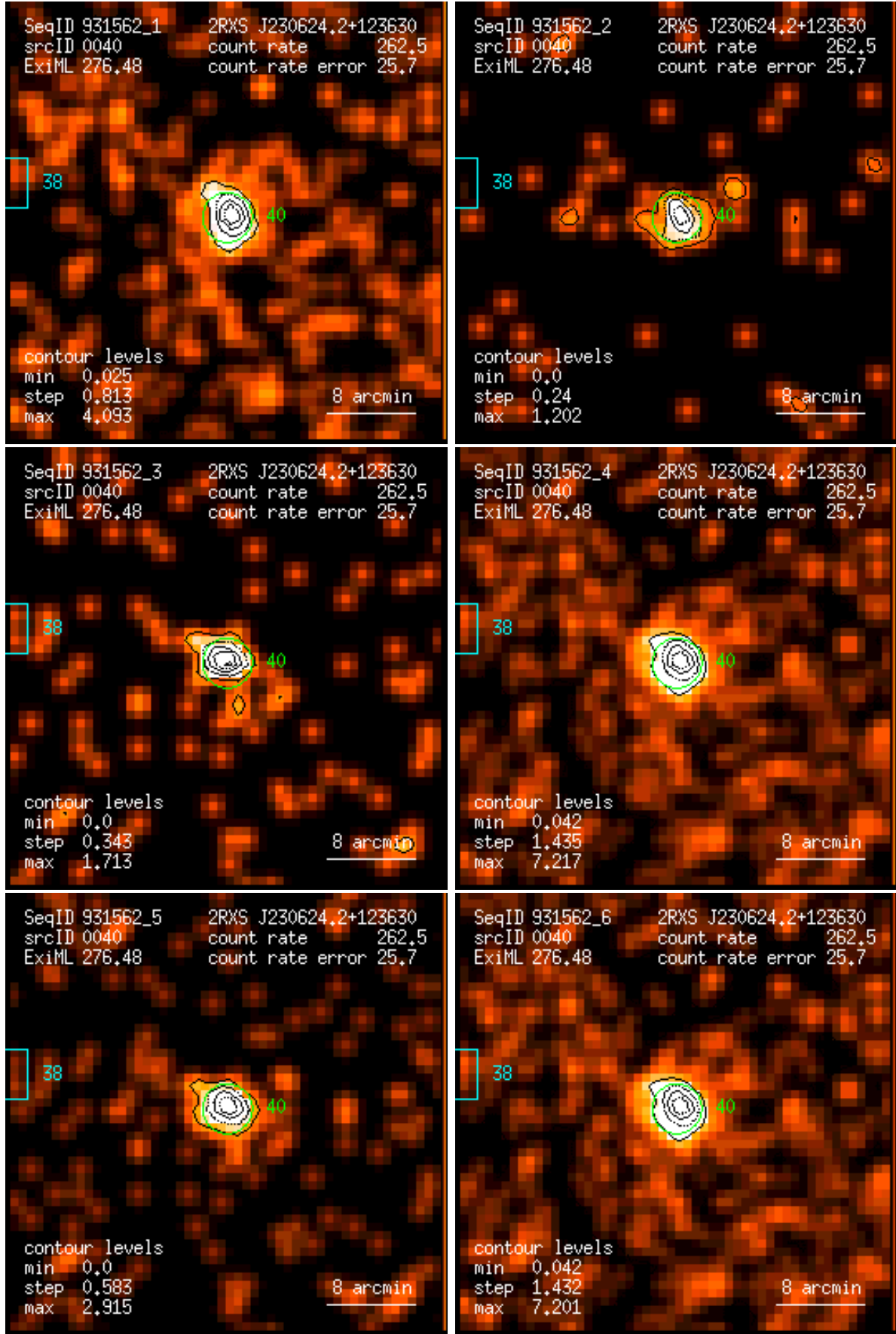
Figure 40: RASS 931562: detection 0040: band rate images, Gaussian filter: (1) PSPC channels 11 – 41, (2) 52 – 90, (3) 91 – 201, (4) 11 – 235, (5) 52 – 201, (6) 11 – 201. Broad band rates in counts/ks. Band rate contour levels in counts/ks/arcmin 2 .
