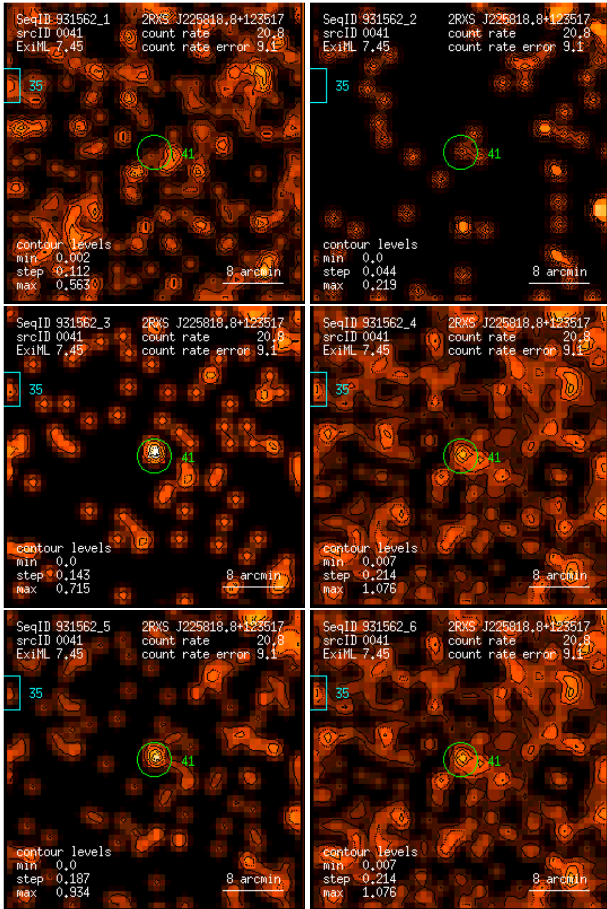
Figure 41: RASS 931562: detection 0041: band rate images, Gaussian filter: (1) PSPC channels 11 – 41, (2) 52 – 90, (3) 91 – 201, (4) 11 – 235, (5) 52 – 201, (6) 11 – 201. Broad band rates in counts/ks. Band rate contour levels in counts/ks/arcmin 2 .
