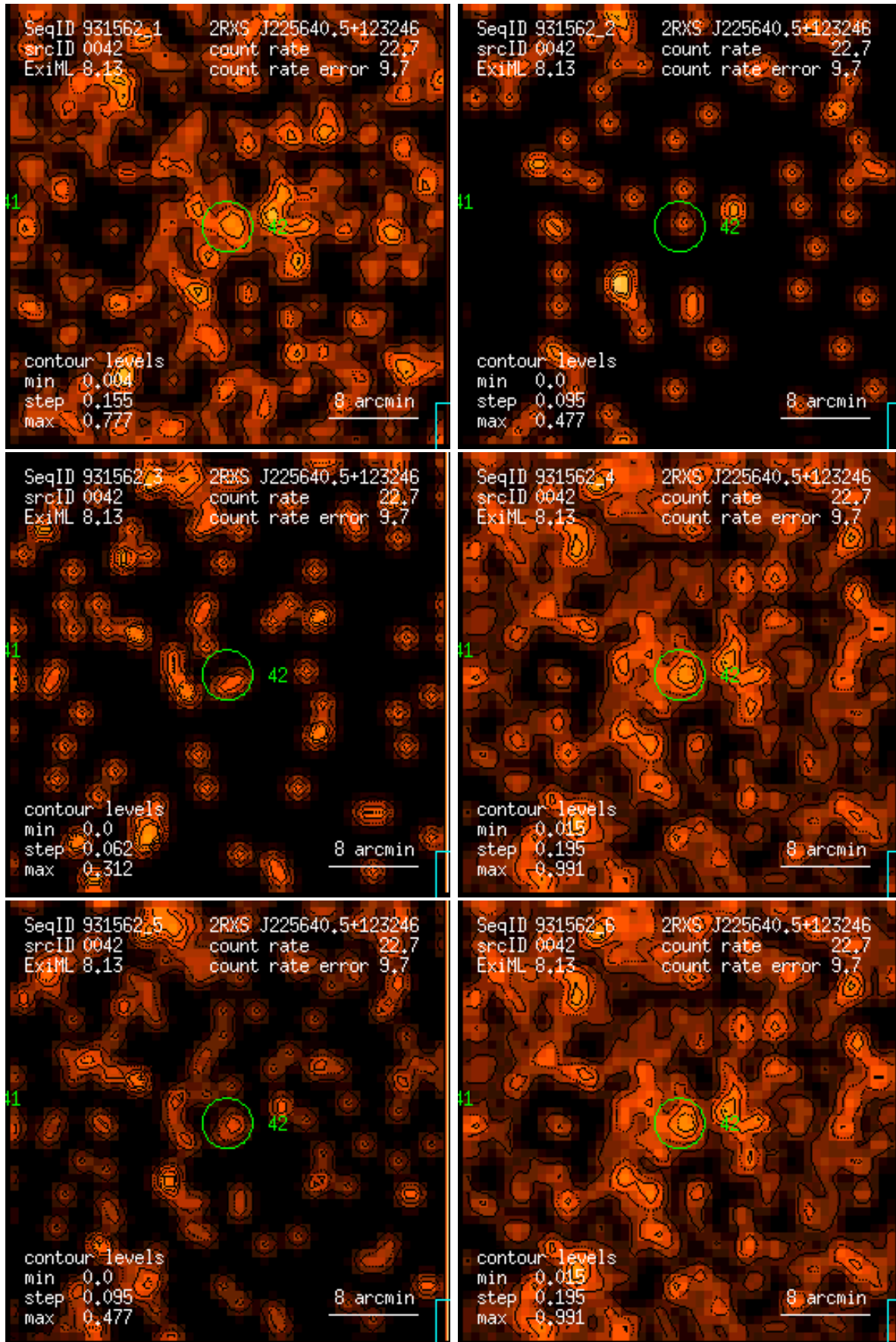
Figure 42: RASS 931562: detection 0042: band rate images, Gaussian filter: (1) PSPC channels 11 – 41, (2) 52 – 90, (3) 91 – 201, (4) 11 – 235, (5) 52 – 201, (6) 11 – 201. Broad band rates in counts/ks. Band rate contour levels in counts/ks/arcmin 2 .
