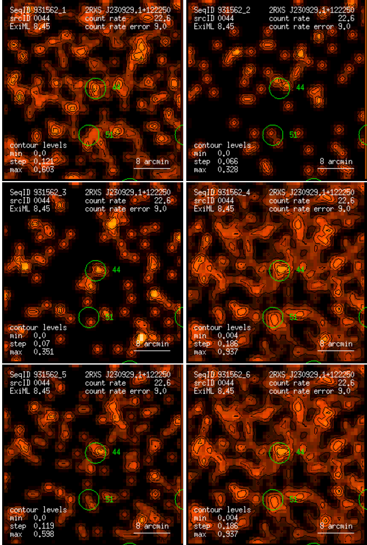
Figure 44: RASS 931562: detection 0044: band rate images, Gaussian filter: (1) PSPC channels 11 – 41, (2) 52 – 90, (3) 91 – 201, (4) 11 – 235, (5) 52 – 201, (6) 11 – 201. Broad band rates in counts/ks. Band rate contour levels in counts/ks/arcmin 2 .
