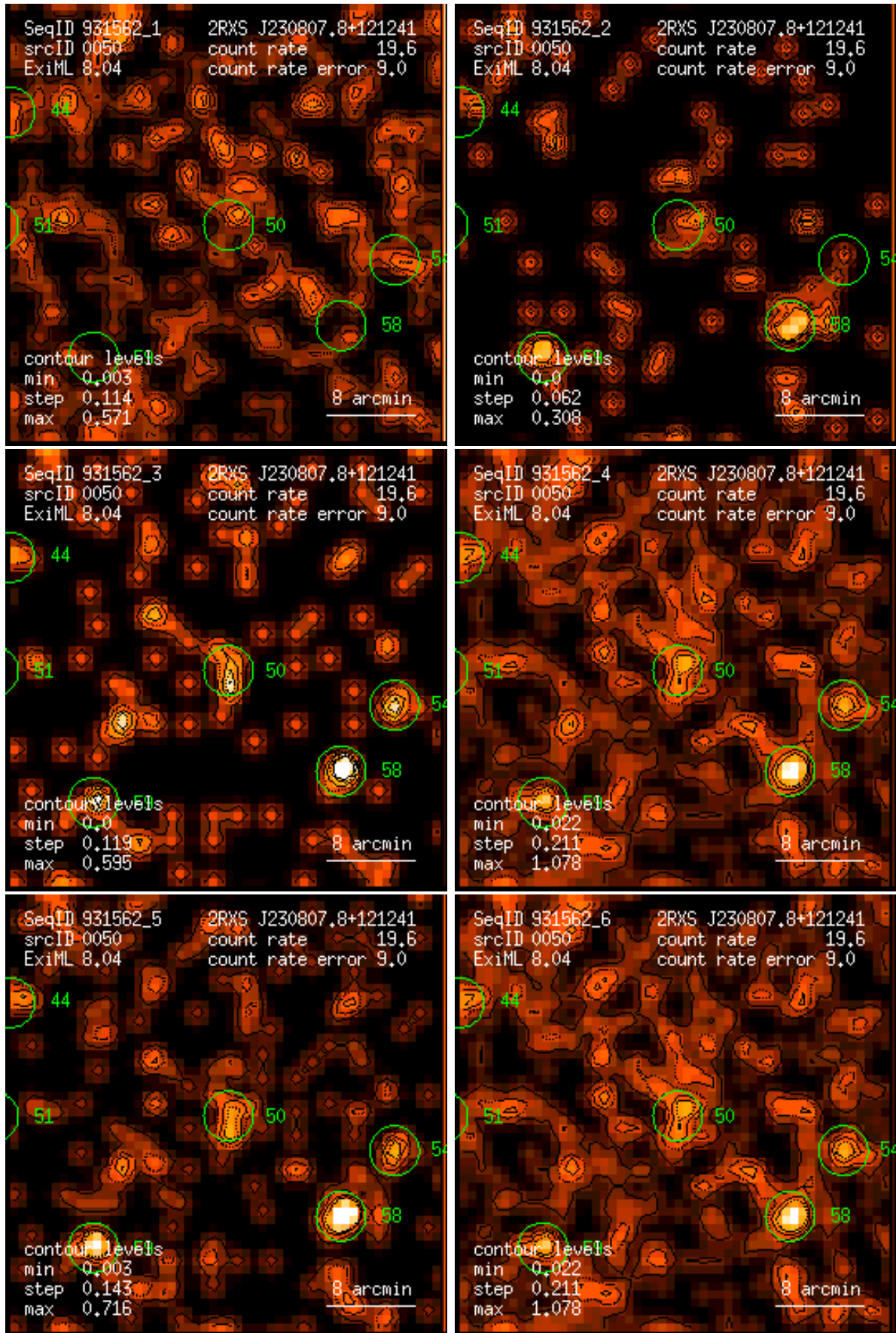
Figure 50: RASS 931562: detection 0050: band rate images, Gaussian filter: (1) PSPC channels 11 – 41, (2) 52 – 90, (3) 91 – 201, (4) 11 – 235, (5) 52 – 201, (6) 11 – 201. Broad band rates in counts/ks. Band rate contour levels in counts/ks/arcmin 2 .
