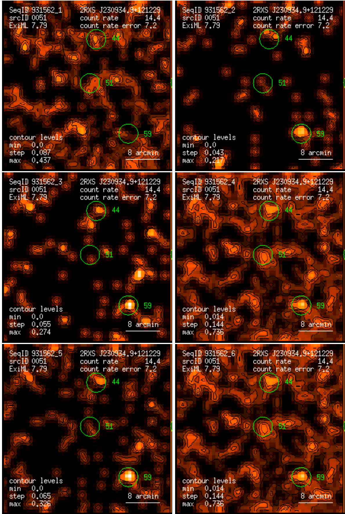
Figure 51: RASS 931562: detection 0051: band rate images, Gaussian filter: (1) PSPC channels 11 – 41, (2) 52 – 90, (3) 91 – 201, (4) 11 – 235, (5) 52 – 201, (6) 11 – 201. Broad band rates in counts/ks. Band rate contour levels in counts/ks/arcmin 2 .
