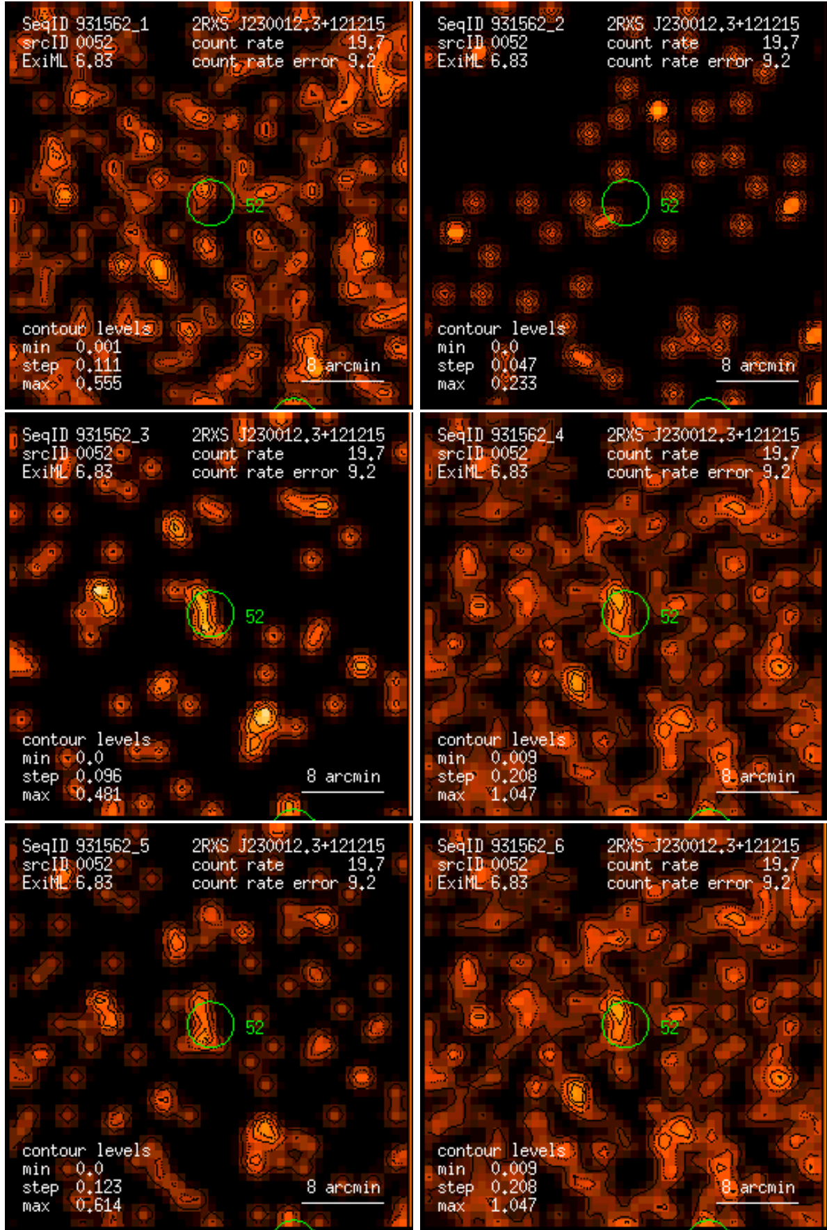
Figure 52: RASS 931562: detection 0052: band rate images, Gaussian filter: (1) PSPC channels 11 – 41, (2) 52 – 90, (3) 91 – 201, (4) 11 – 235, (5) 52 – 201, (6) 11 – 201. Broad band rates in counts/ks. Band rate contour levels in counts/ks/arcmin 2 .
