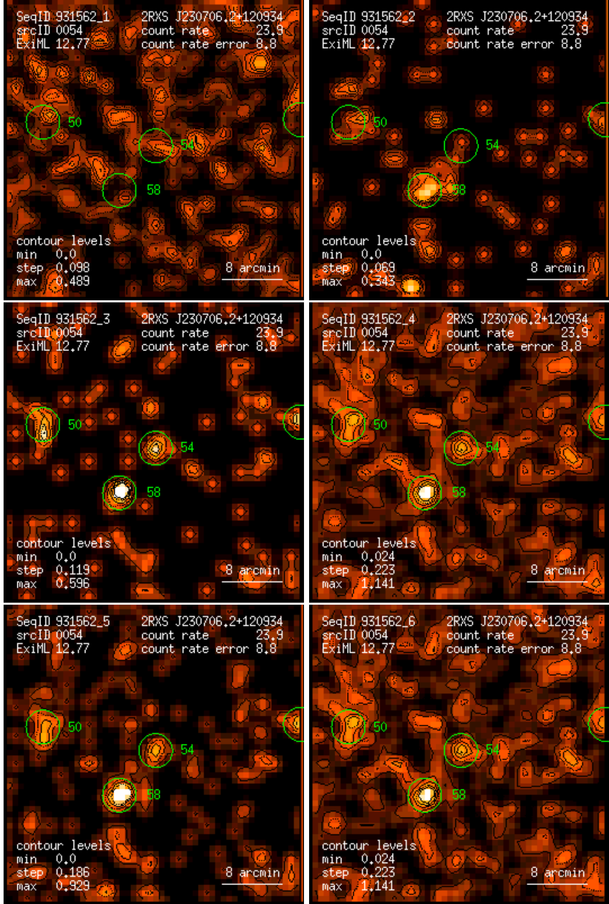
Figure 54: RASS 931562: detection 0054: band rate images, Gaussian filter: (1) PSPC channels 11 – 41, (2) 52 – 90, (3) 91 – 201, (4) 11 – 235, (5) 52 – 201, (6) 11 – 201. Broad band rates in counts/ks. Band rate contour levels in counts/ks/arcmin 2 .
