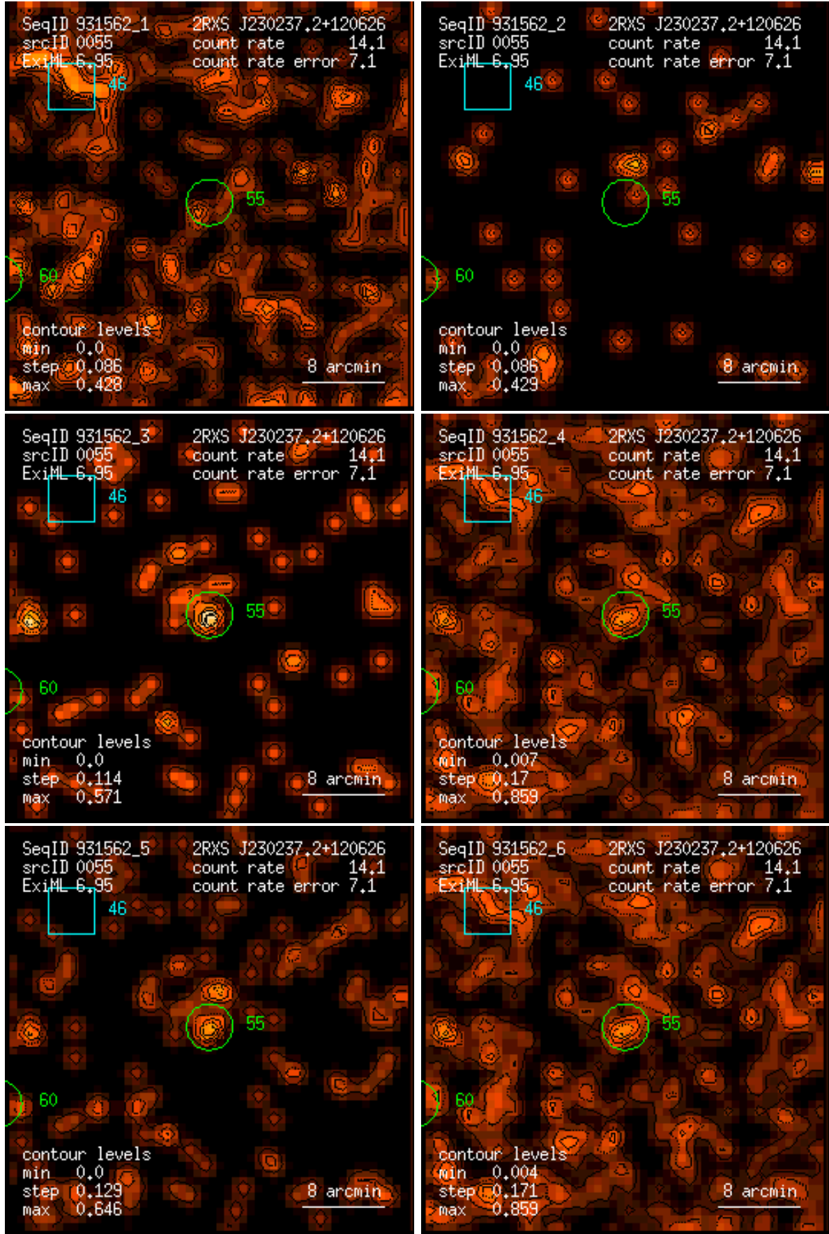
Figure 55: RASS 931562: detection 0055: band rate images, Gaussian filter: (1) PSPC channels 11 – 41, (2) 52 – 90, (3) 91 – 201, (4) 11 – 235, (5) 52 – 201, (6) 11 – 201. Broad band rates in counts/ks. Band rate contour levels in counts/ks/arcmin 2 .
