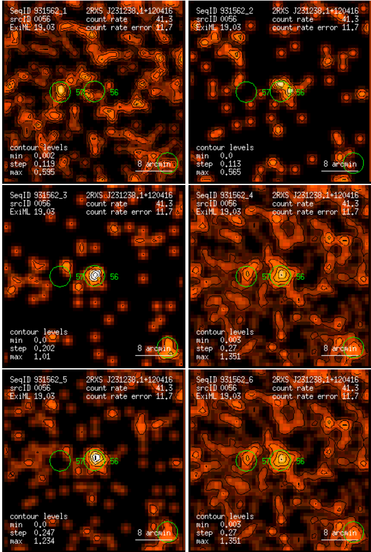
Figure 56: RASS 931562: detection 0056: band rate images, Gaussian filter: (1) PSPC channels 11 – 41, (2) 52 – 90, (3) 91 – 201, (4) 11 – 235, (5) 52 – 201, (6) 11 – 201. Broad band rates in counts/ks. Band rate contour levels in counts/ks/arcmin 2 .
