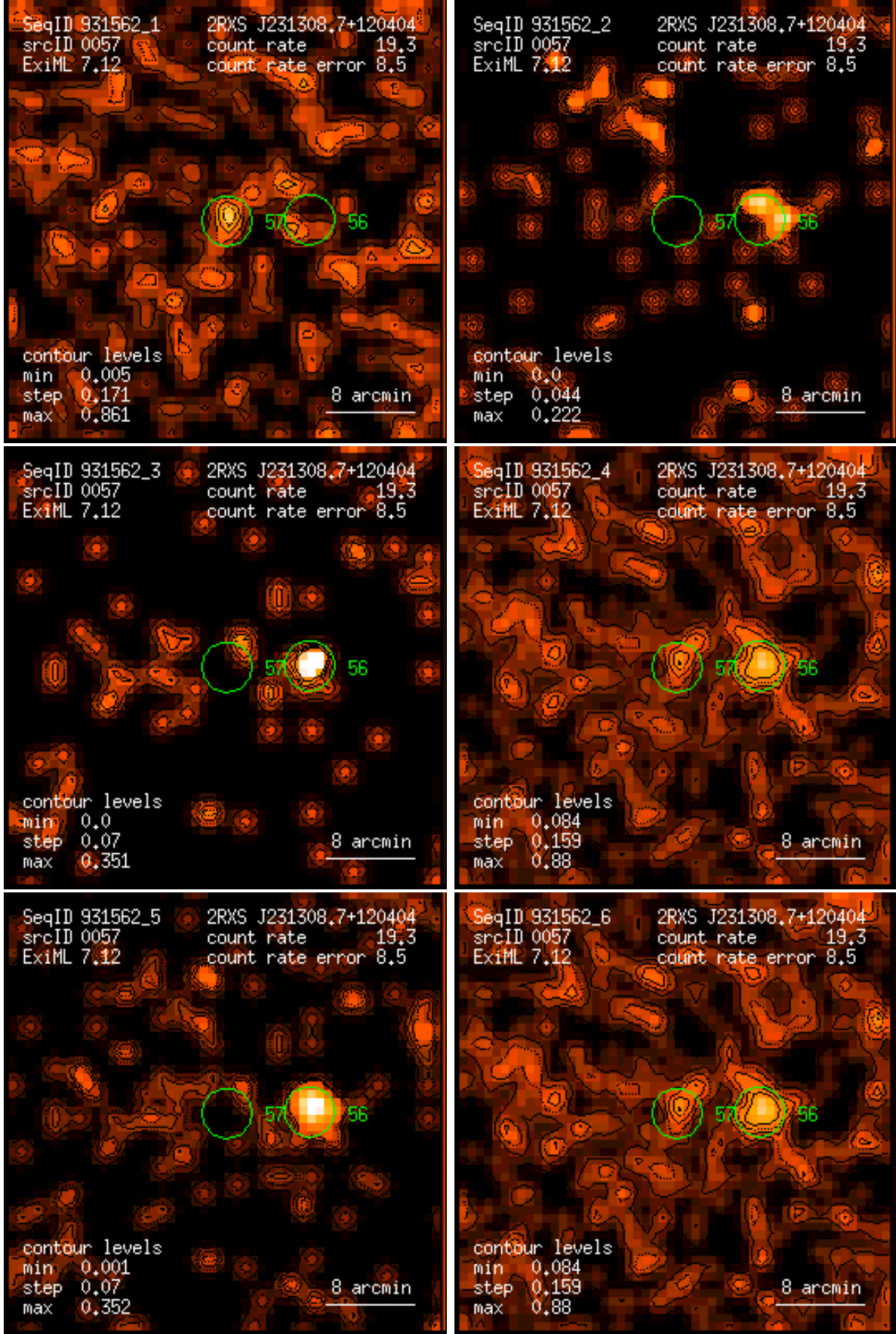
Figure 57: RASS 931562: detection 0057: band rate images, Gaussian filter: (1) PSPC channels 11 – 41, (2) 52 – 90, (3) 91 – 201, (4) 11 – 235, (5) 52 – 201, (6) 11 – 201. Broad band rates in counts/ks. Band rate contour levels in counts/ks/arcmin 2 .
