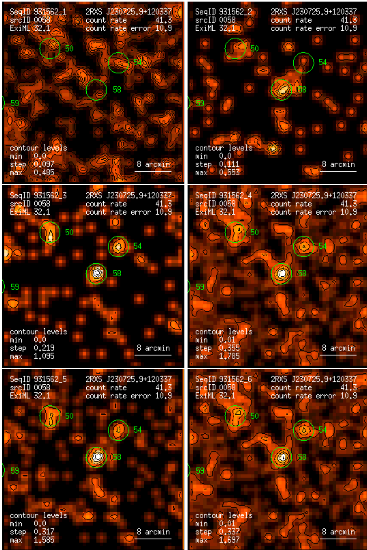
Figure 58: RASS 931562: detection 0058: band rate images, Gaussian filter: (1) PSPC channels 11 – 41, (2) 52 – 90, (3) 91 – 201, (4) 11 – 235, (5) 52 – 201, (6) 11 – 201. Broad band rates in counts/ks. Band rate contour levels in counts/ks/arcmin 2 .
