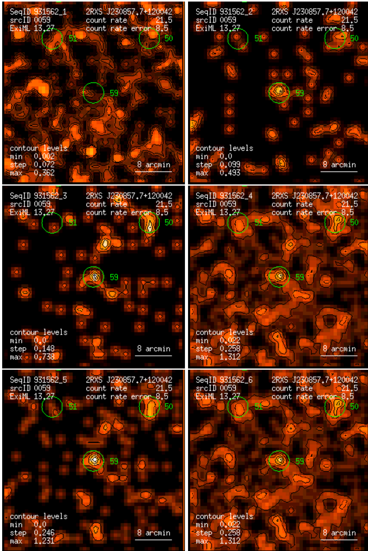
Figure 59: RASS 931562: detection 0059: band rate images, Gaussian filter: (1) PSPC channels 11 – 41, (2) 52 – 90, (3) 91 – 201, (4) 11 – 235, (5) 52 – 201, (6) 11 – 201. Broad band rates in counts/ks. Band rate contour levels in counts/ks/arcmin 2 .
