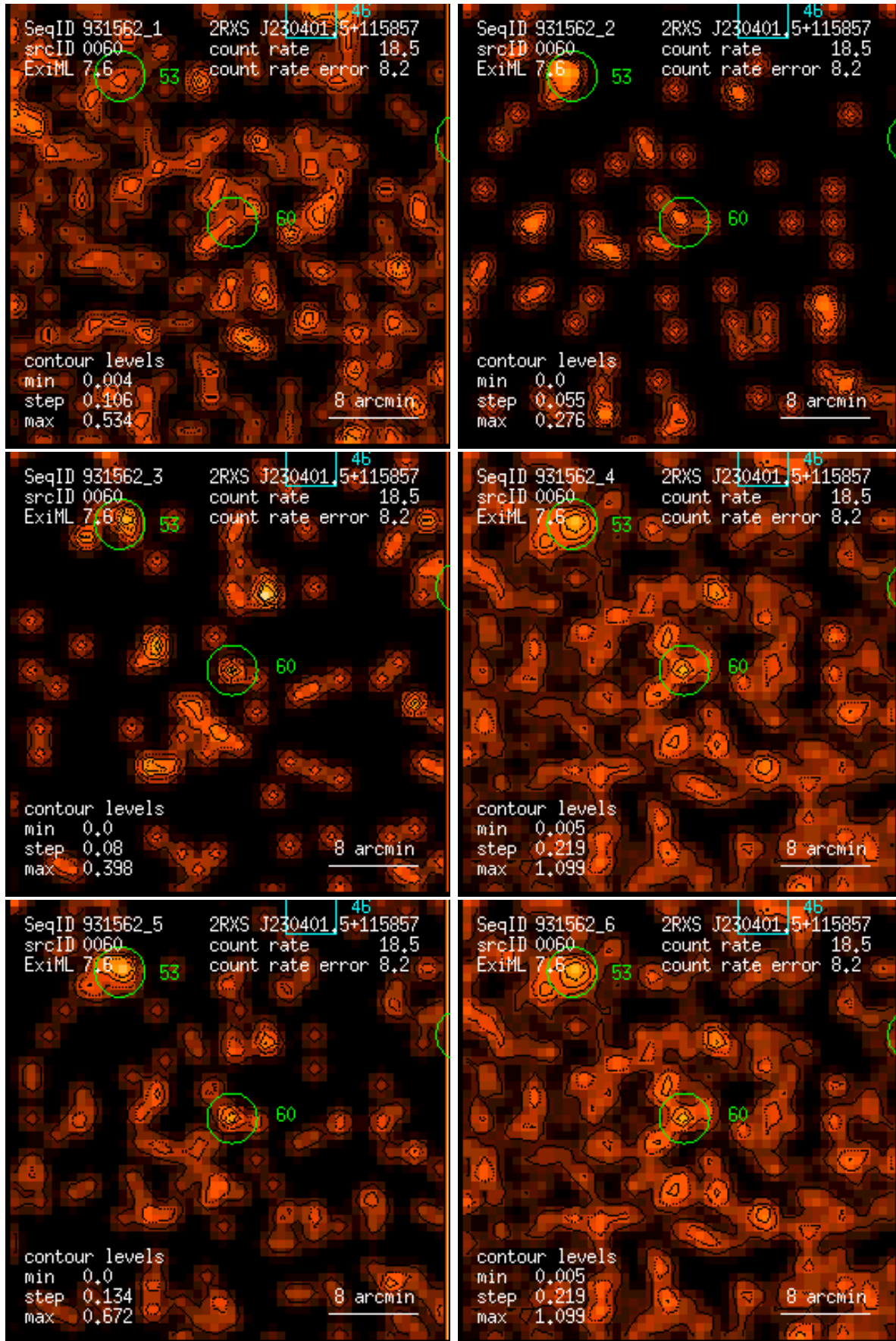
Figure 60: RASS 931562: detection 0060: band rate images, Gaussian filter: (1) PSPC channels 11 – 41, (2) 52 – 90, (3) 91 – 201, (4) 11 – 235, (5) 52 – 201, (6) 11 – 201. Broad band rates in counts/ks. Band rate contour levels in counts/ks/arcmin 2 .
