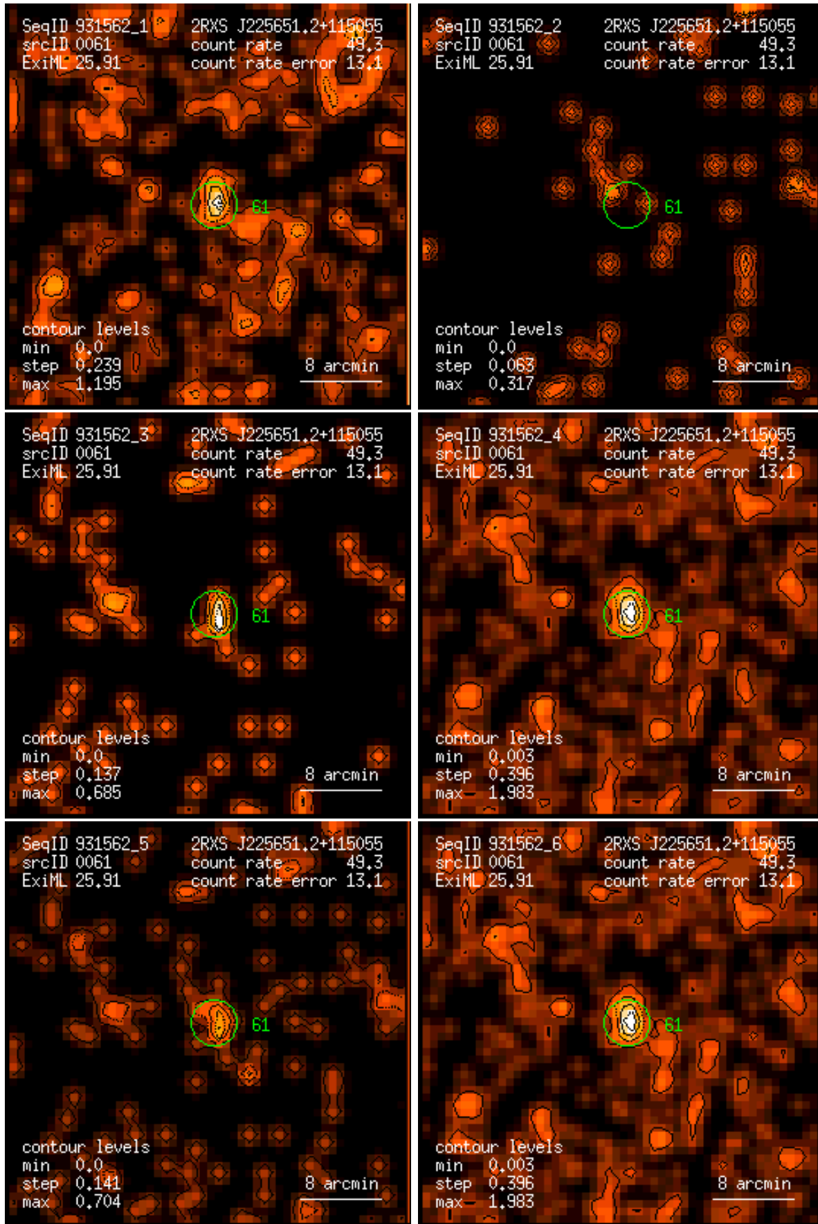
Figure 61: RASS 931562: detection 0061: band rate images, Gaussian filter: (1) PSPC channels 11 – 41, (2) 52 – 90, (3) 91 – 201, (4) 11 – 235, (5) 52 – 201, (6) 11 – 201. Broad band rates in counts/ks. Band rate contour levels in counts/ks/arcmin 2 .
