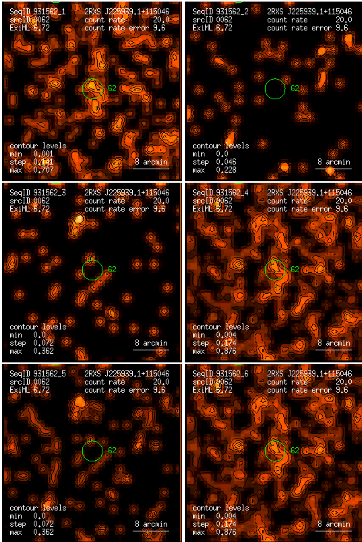
Figure 62: RASS 931562: detection 0062: band rate images, Gaussian filter: (1) PSPC channels 11 – 41, (2) 52 – 90, (3) 91 – 201, (4) 11 – 235, (5) 52 – 201, (6) 11 – 201. Broad band rates in counts/ks. Band rate contour levels in counts/ks/arcmin 2 .
