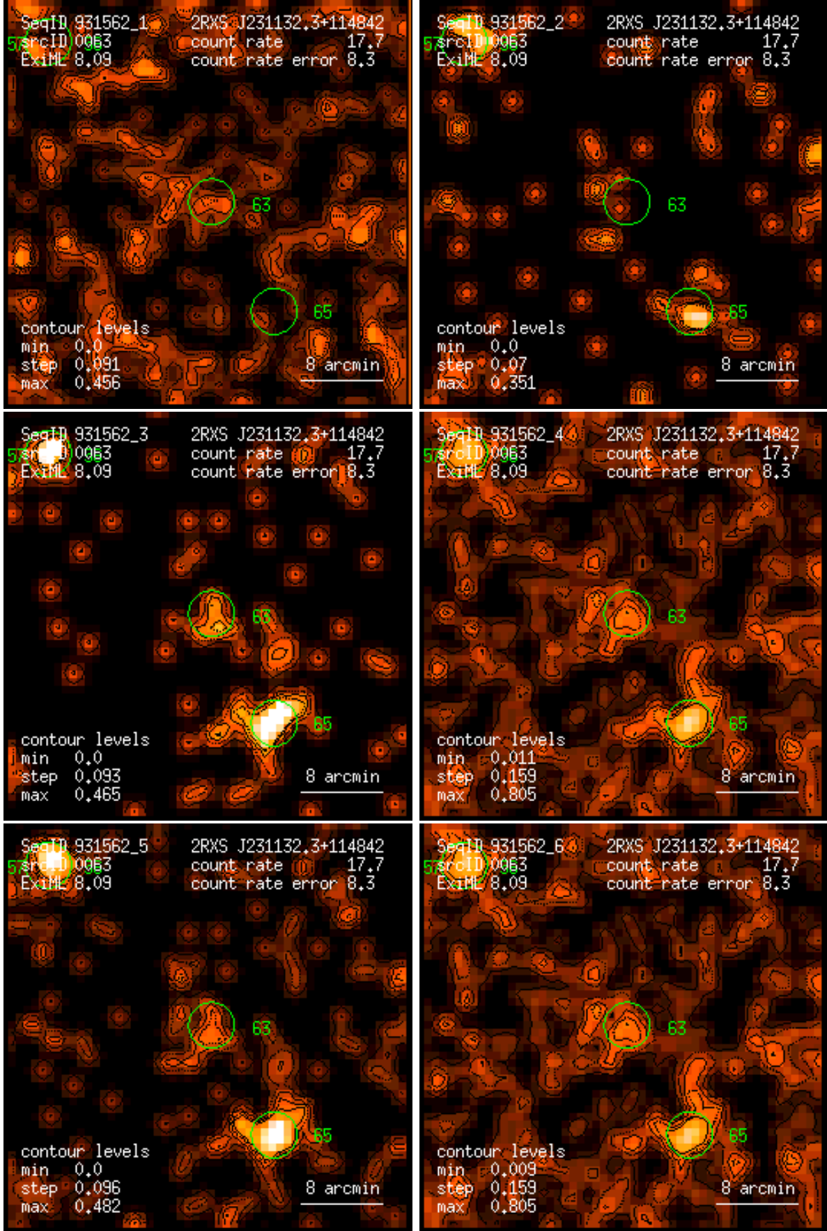
Figure 63: RASS 931562: detection 0063: band rate images, Gaussian filter: (1) PSPC channels 11 – 41, (2) 52 – 90, (3) 91 – 201, (4) 11 – 235, (5) 52 – 201, (6) 11 – 201. Broad band rates in counts/ks. Band rate contour levels in counts/ks/arcmin 2 .
