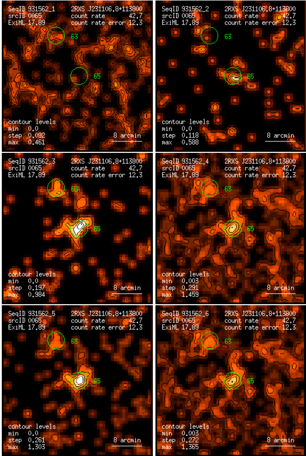
Figure 65: RASS 931562: detection 0065: band rate images, Gaussian filter: (1) PSPC channels 11 – 41, (2) 52 – 90, (3) 91 – 201, (4) 11 – 235, (5) 52 – 201, (6) 11 – 201. Broad band rates in counts/ks. Band rate contour levels in counts/ks/arcmin 2 .
