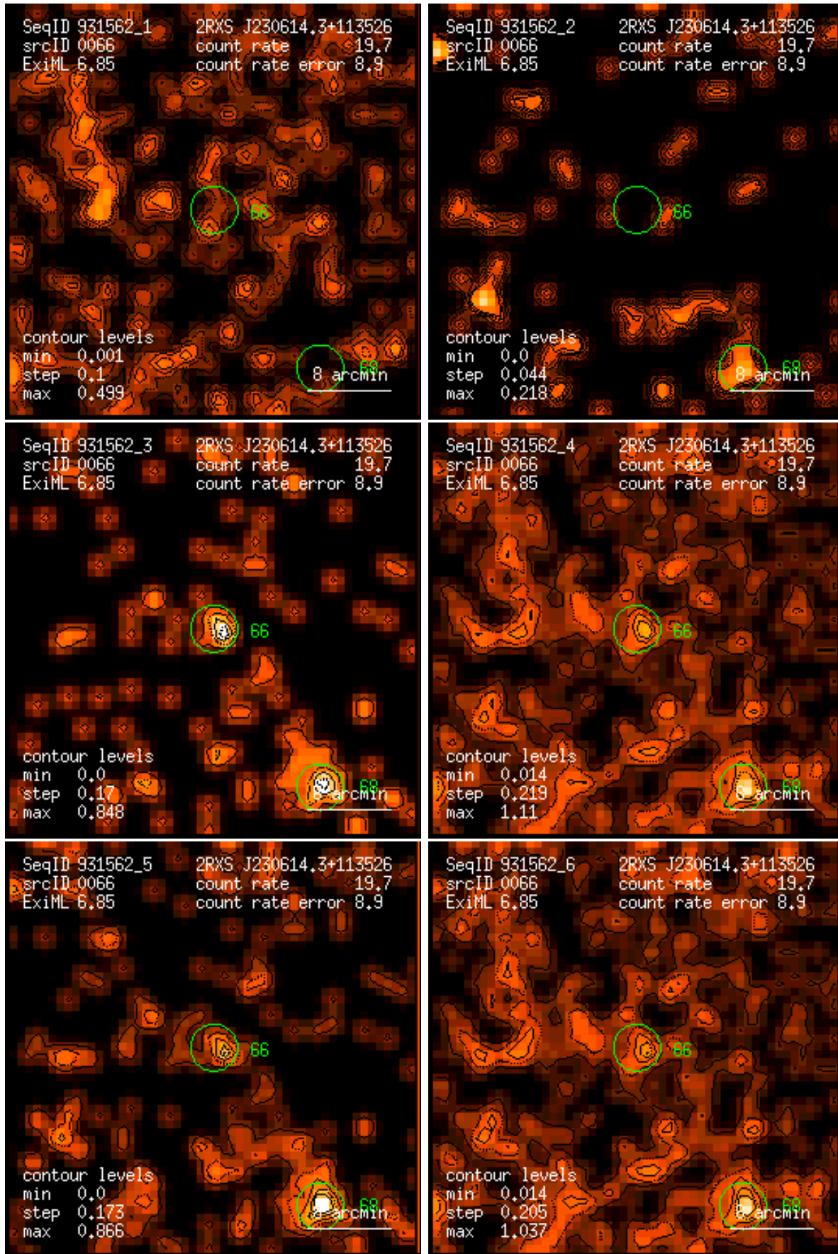
Figure 66: RASS 931562: detection 0066: band rate images, Gaussian filter: (1) PSPC channels 11 – 41, (2) 52 – 90, (3) 91 – 201, (4) 11 – 235, (5) 52 – 201, (6) 11 – 201. Broad band rates in counts/ks. Band rate contour levels in counts/ks/arcmin 2 .
