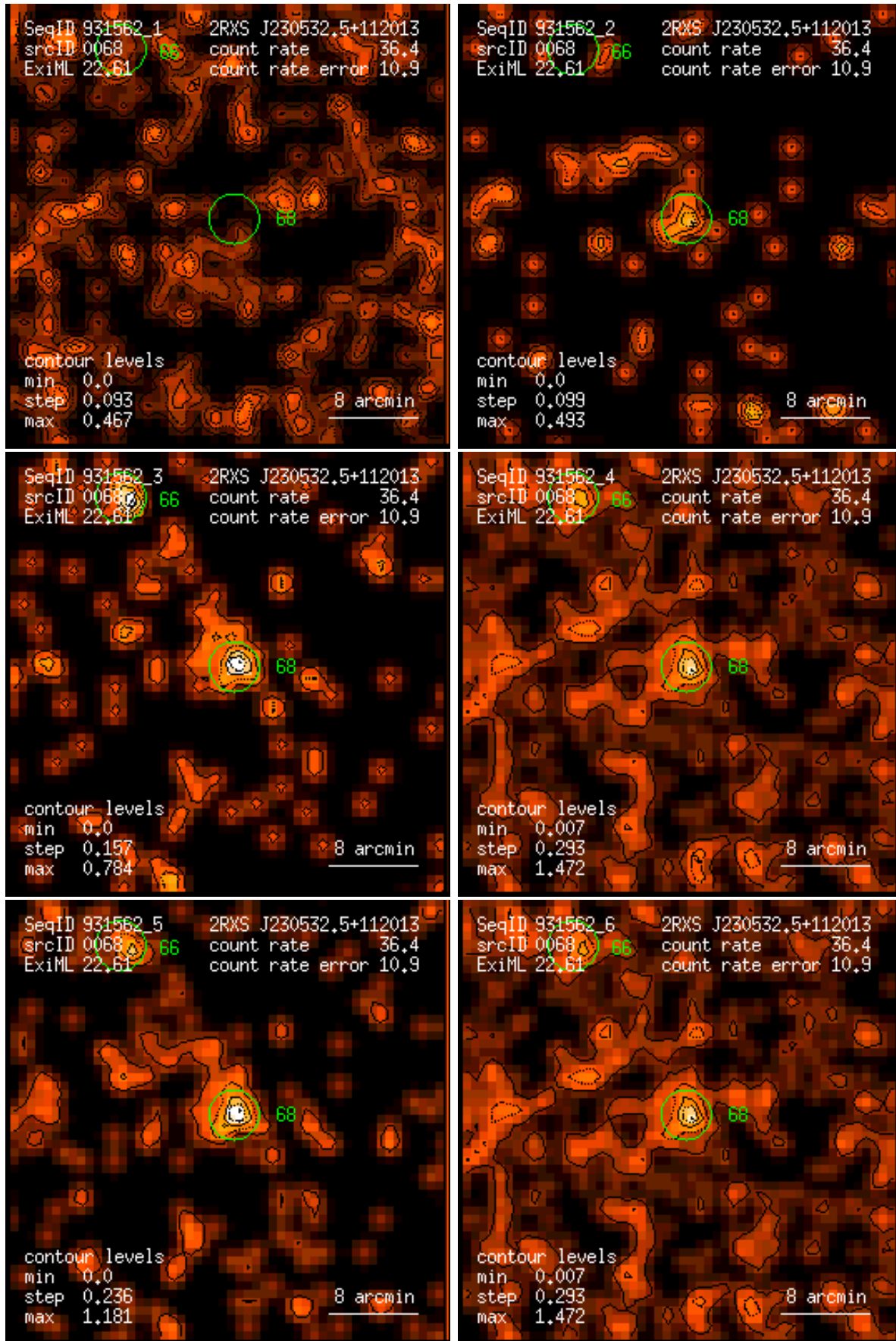
Figure 68: RASS 931562: detection 0068: band rate images, Gaussian filter: (1) PSPC channels 11 – 41, (2) 52 – 90, (3) 91 – 201, (4) 11 – 235, (5) 52 – 201, (6) 11 – 201. Broad band rates in counts/ks. Band rate contour levels in counts/ks/arcmin 2 .
