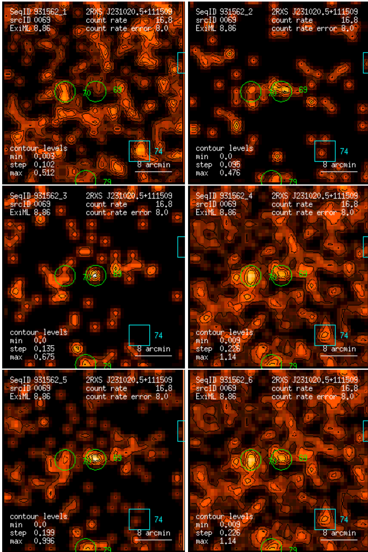
Figure 69: RASS 931562: detection 0069: band rate images, Gaussian filter: (1) PSPC channels 11 – 41, (2) 52 – 90, (3) 91 – 201, (4) 11 – 235, (5) 52 – 201, (6) 11 – 201. Broad band rates in counts/ks. Band rate contour levels in counts/ks/arcmin 2 .
