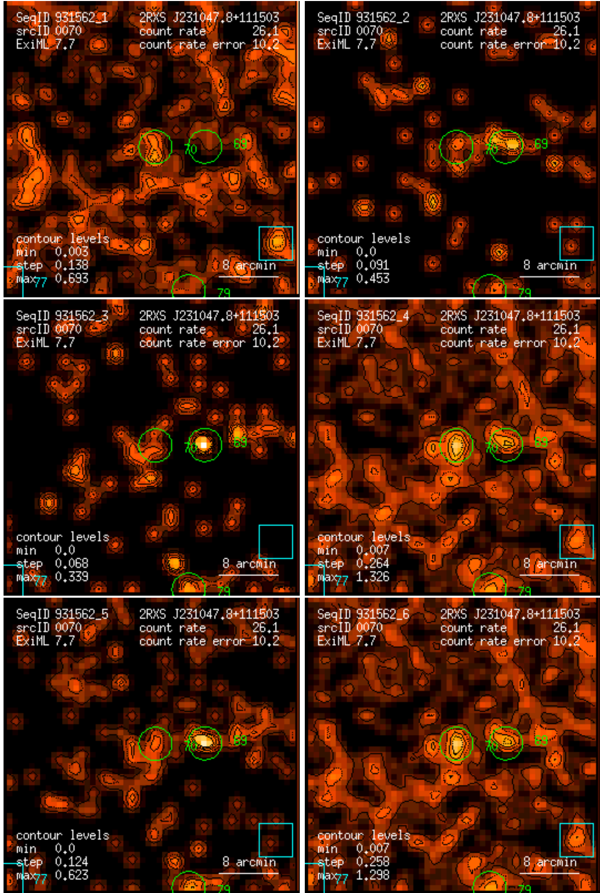
Figure 70: RASS 931562: detection 0070: band rate images, Gaussian filter: (1) PSPC channels 11 – 41, (2) 52 – 90, (3) 91 – 201, (4) 11 – 235, (5) 52 – 201, (6) 11 – 201. Broad band rates in counts/ks. Band rate contour levels in counts/ks/arcmin 2 .
