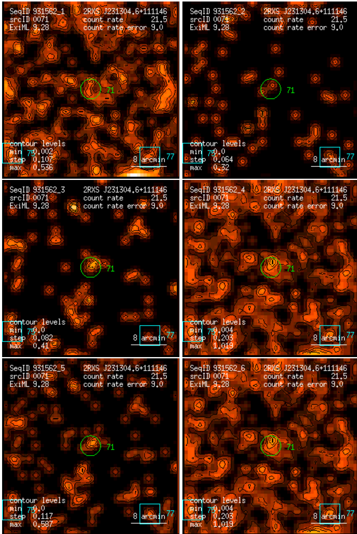
Figure 71: RASS 931562: detection 0071: band rate images, Gaussian filter: (1) PSPC channels 11 – 41, (2) 52 – 90, (3) 91 – 201, (4) 11 – 235, (5) 52 – 201, (6) 11 – 201. Broad band rates in counts/ks. Band rate contour levels in counts/ks/arcmin 2 .
