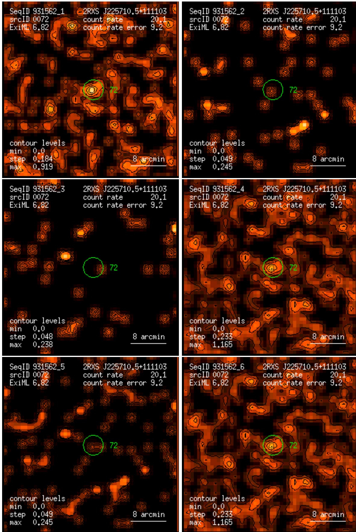
Figure 72: RASS 931562: detection 0072: band rate images, Gaussian filter: (1) PSPC channels 11 – 41, (2) 52 – 90, (3) 91 – 201, (4) 11 – 235, (5) 52 – 201, (6) 11 – 201. Broad band rates in counts/ks. Band rate contour levels in counts/ks/arcmin 2 .
