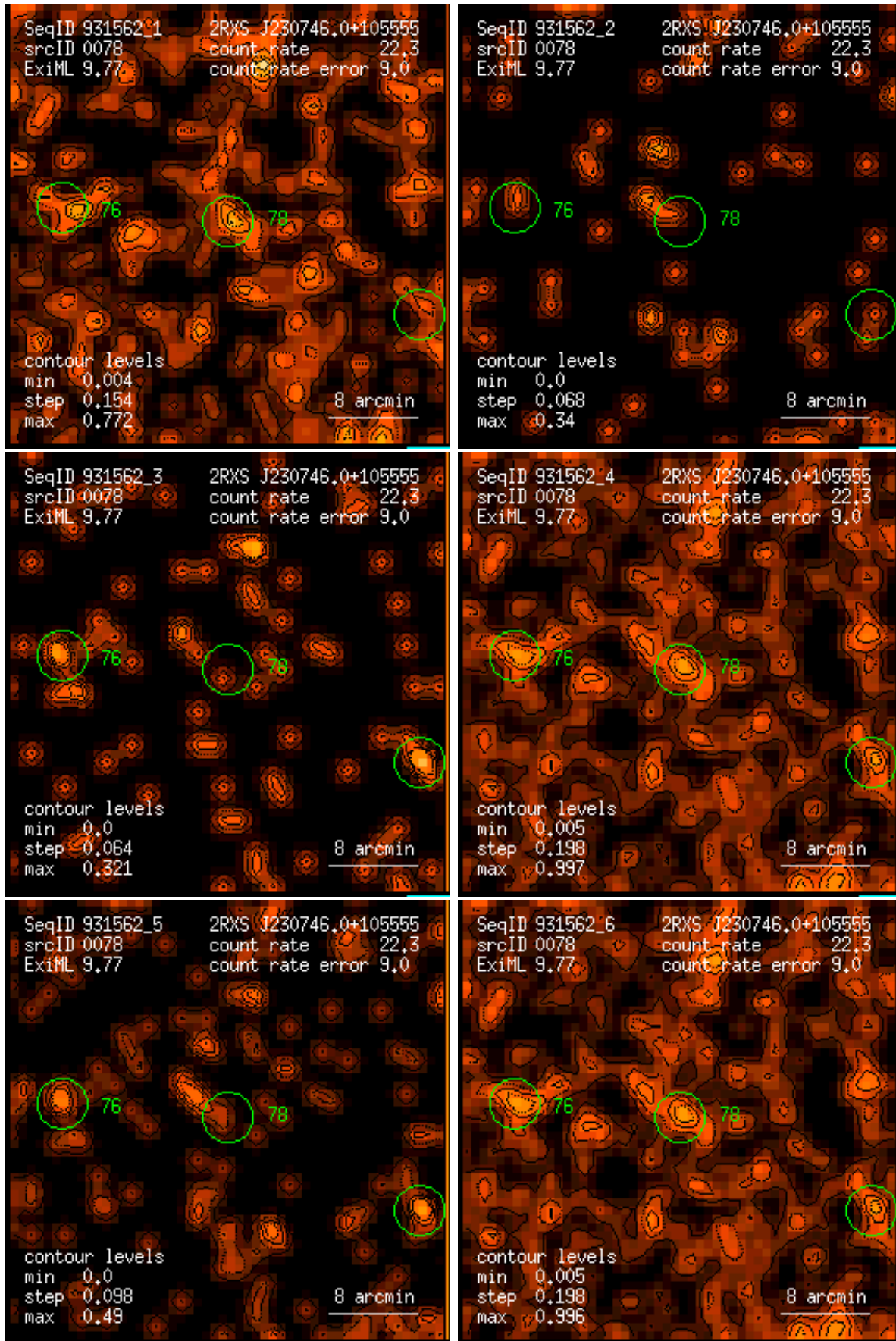
Figure 78: RASS 931562: detection 0078: band rate images, Gaussian filter: (1) PSPC channels 11 – 41, (2) 52 – 90, (3) 91 – 201, (4) 11 – 235, (5) 52 – 201, (6) 11 – 201. Broad band rates in counts/ks. Band rate contour levels in counts/ks/arcmin 2 .
