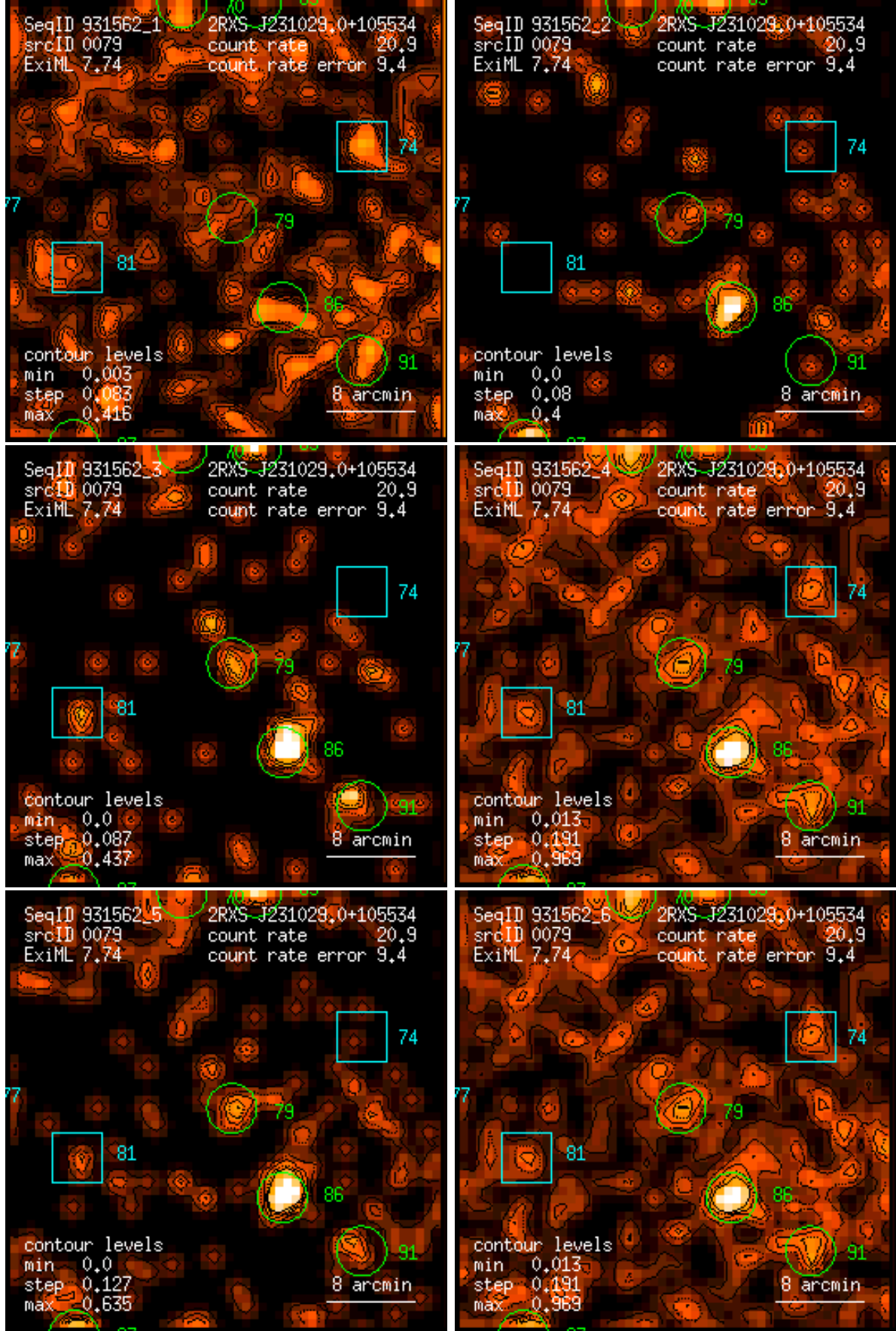
Figure 79: RASS 931562: detection 0079: band rate images, Gaussian filter: (1) PSPC channels 11 – 41, (2) 52 – 90, (3) 91 – 201, (4) 11 – 235, (5) 52 – 201, (6) 11 – 201. Broad band rates in counts/ks. Band rate contour levels in counts/ks/arcmin 2 .
