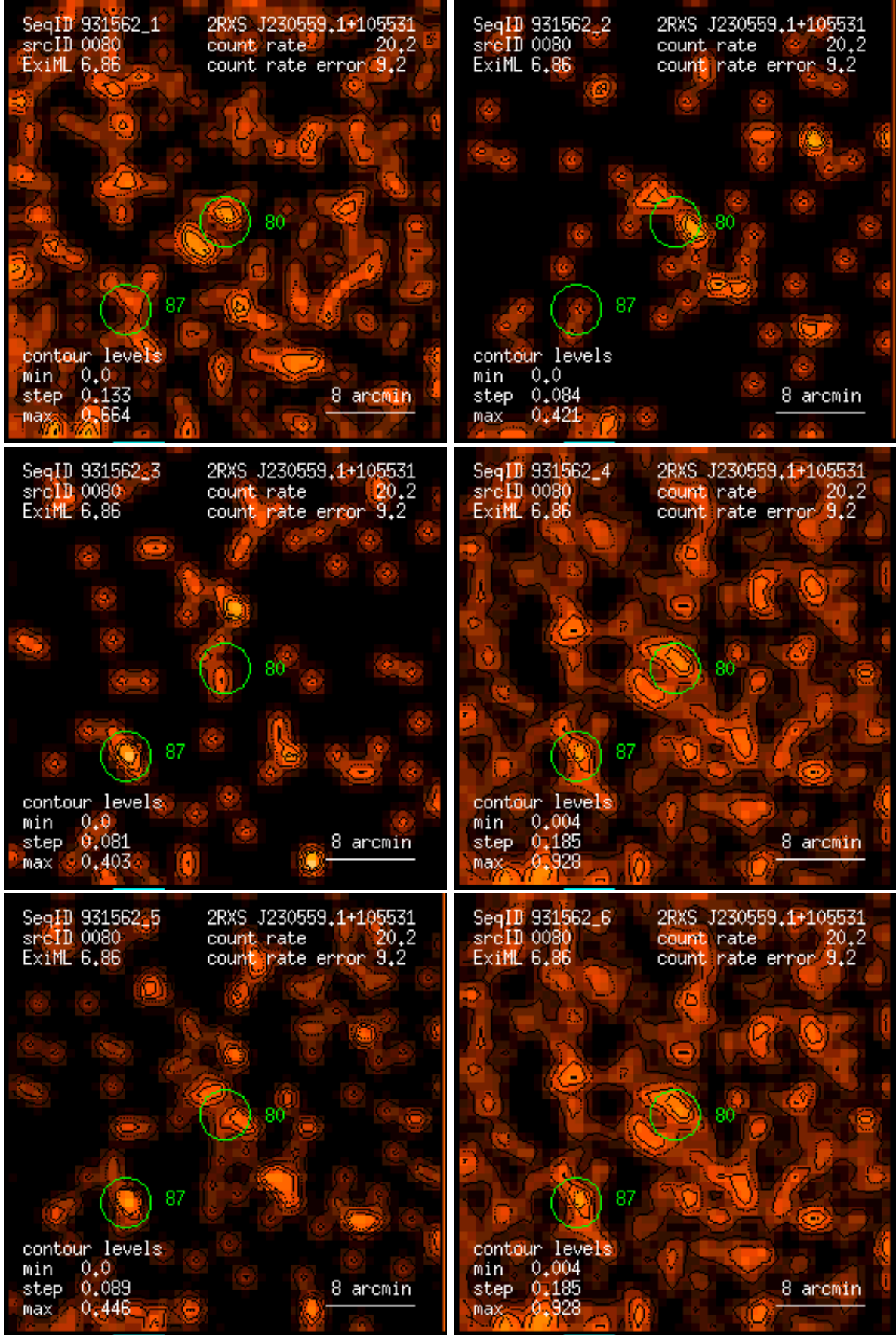
Figure 80: RASS 931562: detection 0080: band rate images, Gaussian filter: (1) PSPC channels 11 – 41, (2) 52 – 90, (3) 91 – 201, (4) 11 – 235, (5) 52 – 201, (6) 11 – 201. Broad band rates in counts/ks. Band rate contour levels in counts/ks/arcmin 2 .
