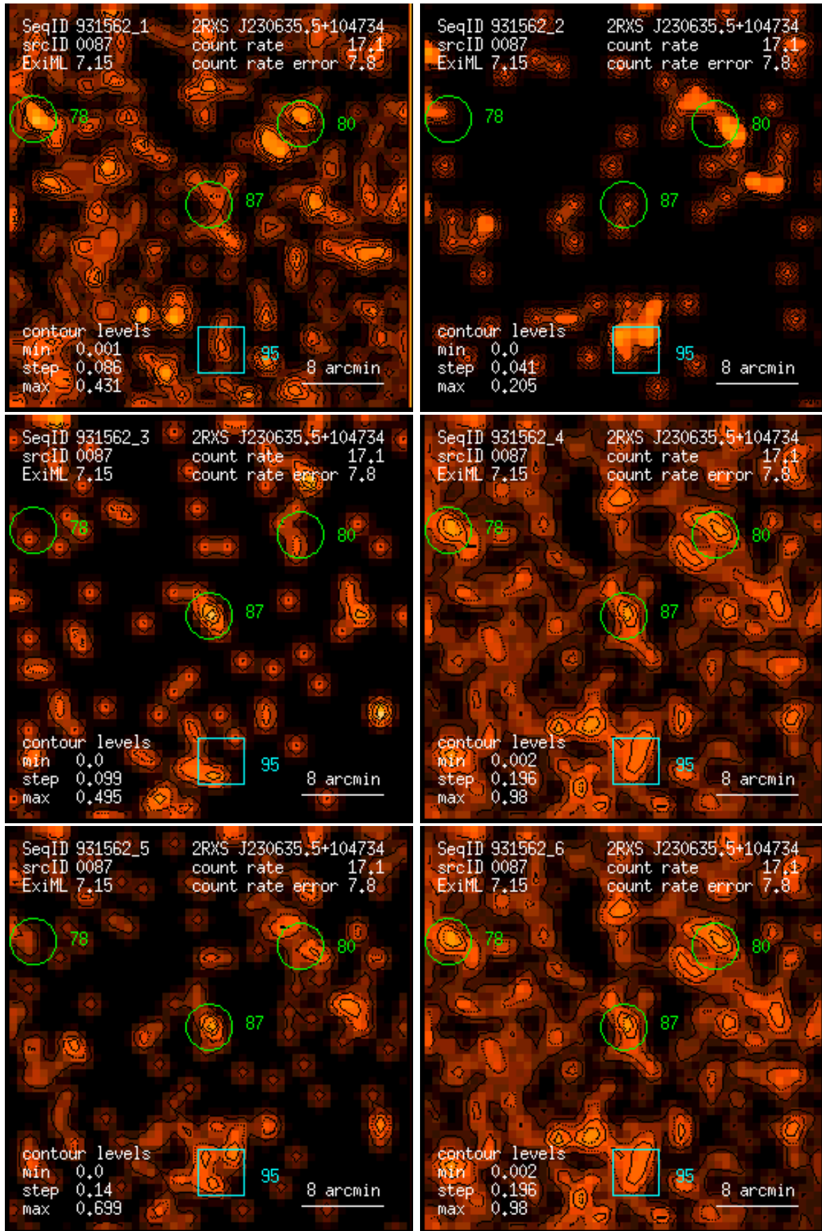
Figure 87: RASS 931562: detection 0087: band rate images, Gaussian filter: (1) PSPC channels 11 – 41, (2) 52 – 90, (3) 91 – 201, (4) 11 – 235, (5) 52 – 201, (6) 11 – 201. Broad band rates in counts/ks. Band rate contour levels in counts/ks/arcmin 2 .
