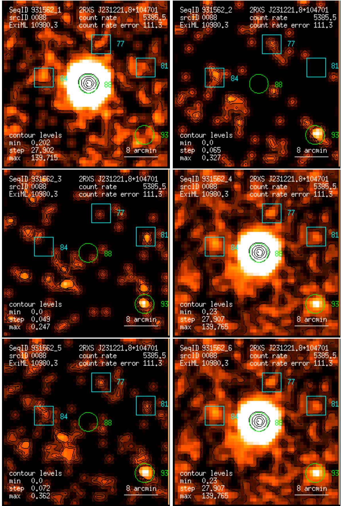
Figure 88: RASS 931562: detection 0088: band rate images, Gaussian filter: (1) PSPC channels 11 – 41, (2) 52 – 90, (3) 91 – 201, (4) 11 – 235, (5) 52 – 201, (6) 11 – 201. Broad band rates in counts/ks. Band rate contour levels in counts/ks/arcmin 2 .
