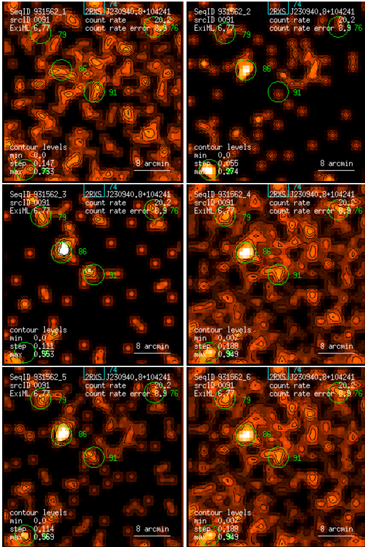
Figure 91: RASS 931562: detection 0091: band rate images, Gaussian filter: (1) PSPC channels 11 – 41, (2) 52 – 90, (3) 91 – 201, (4) 11 – 235, (5) 52 – 201, (6) 11 – 201. Broad band rates in counts/ks. Band rate contour levels in counts/ks/arcmin 2 .
