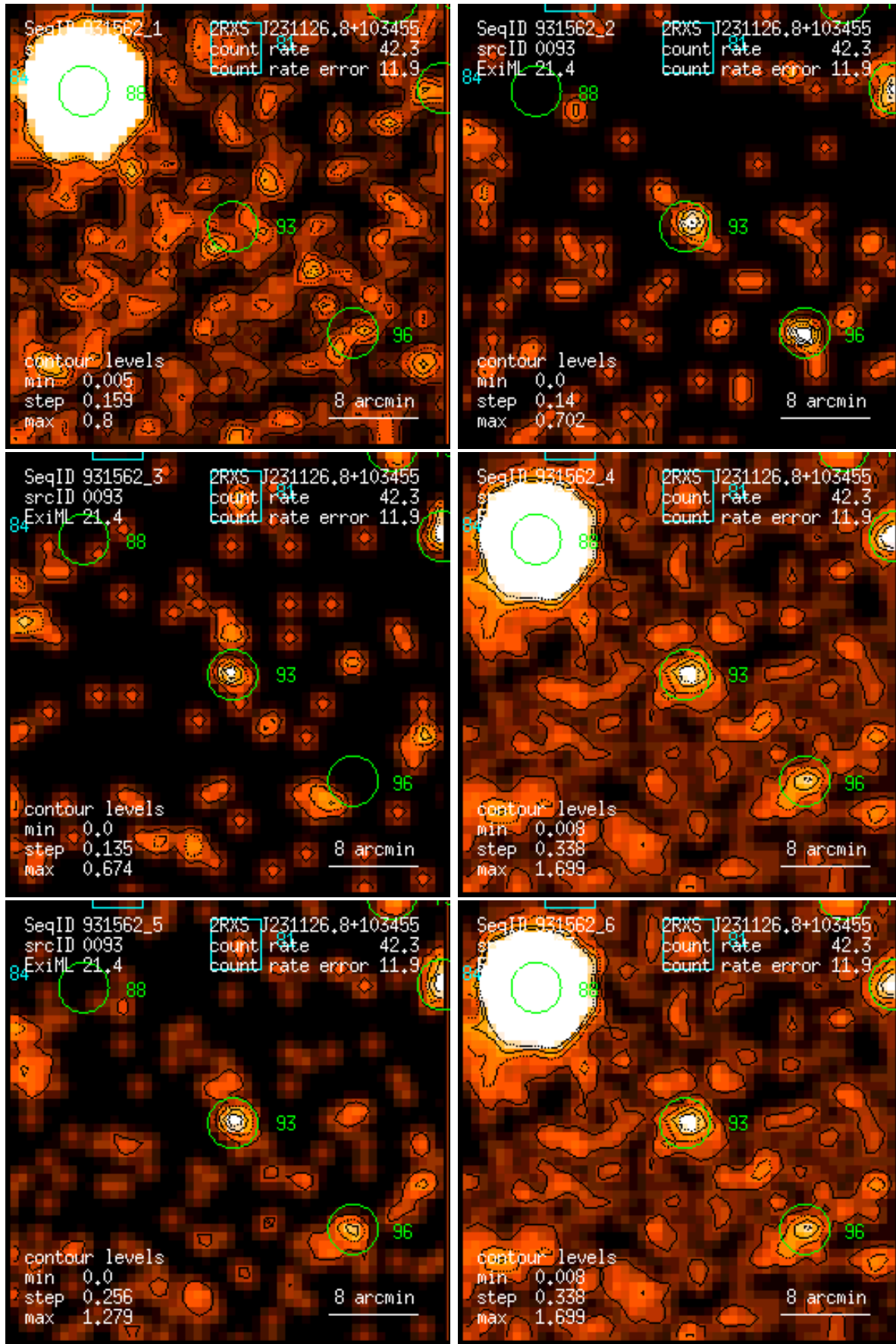
Figure 93: RASS 931562: detection 0093: band rate images, Gaussian filter: (1) PSPC channels 11 – 41, (2) 52 – 90, (3) 91 – 201, (4) 11 – 235, (5) 52 – 201, (6) 11 – 201. Broad band rates in counts/ks. Band rate contour levels in counts/ks/arcmin 2 .
