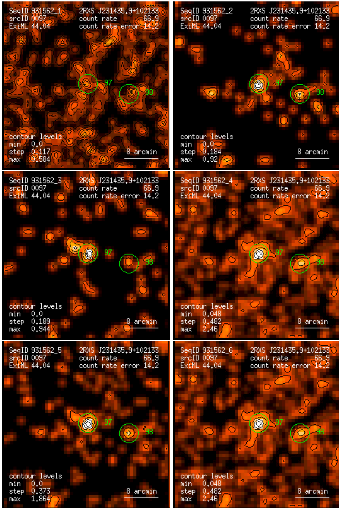
Figure 97: RASS 931562: detection 0097: band rate images, Gaussian filter: (1) PSPC channels 11 – 41, (2) 52 – 90, (3) 91 – 201, (4) 11 – 235, (5) 52 – 201, (6) 11 – 201. Broad band rates in counts/ks. Band rate contour levels in counts/ks/arcmin 2 .
