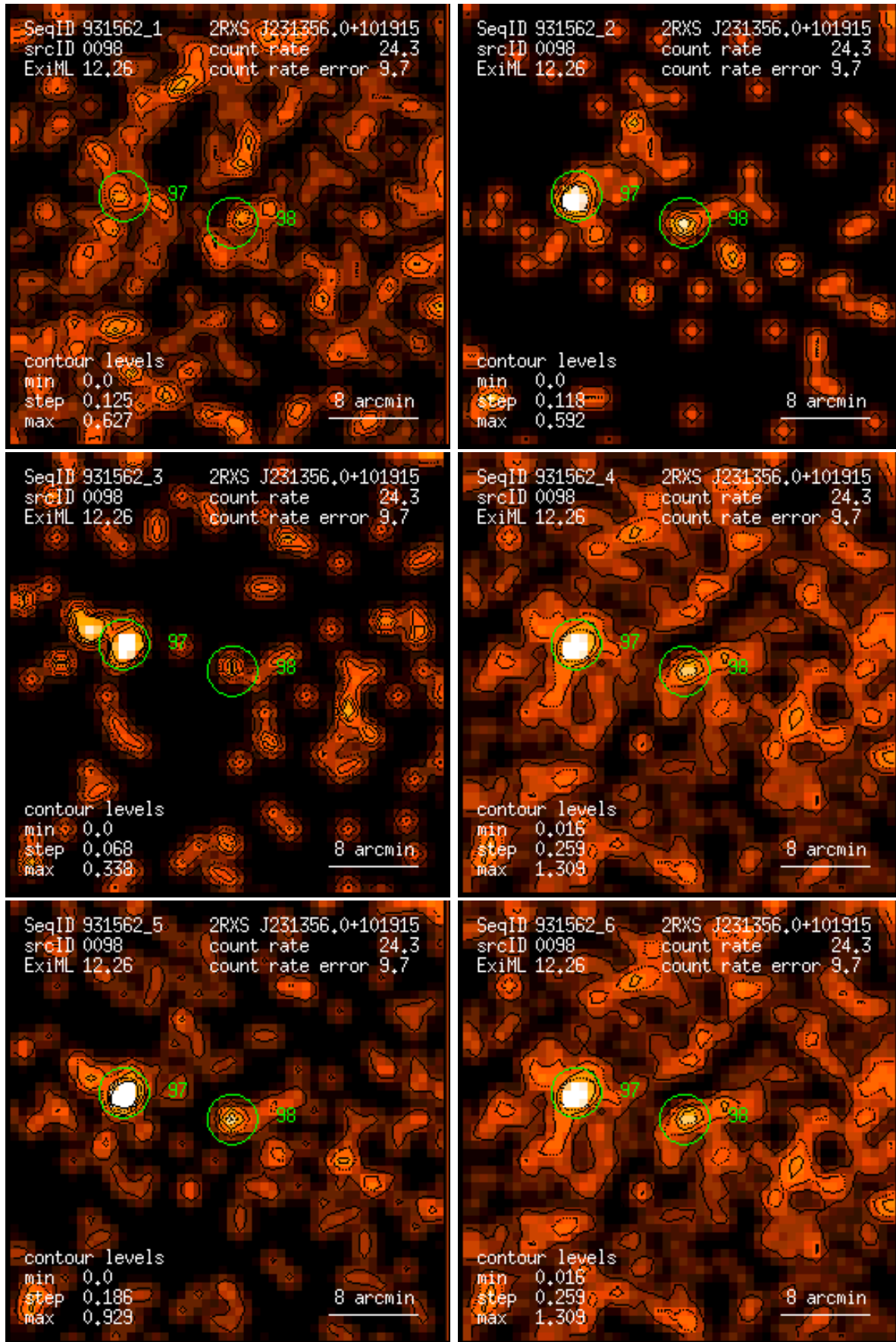
Figure 98: RASS 931562: detection 0098: band rate images, Gaussian filter: (1) PSPC channels 11 – 41, (2) 52 – 90, (3) 91 – 201, (4) 11 – 235, (5) 52 – 201, (6) 11 – 201. Broad band rates in counts/ks. Band rate contour levels in counts/ks/arcmin 2 .
