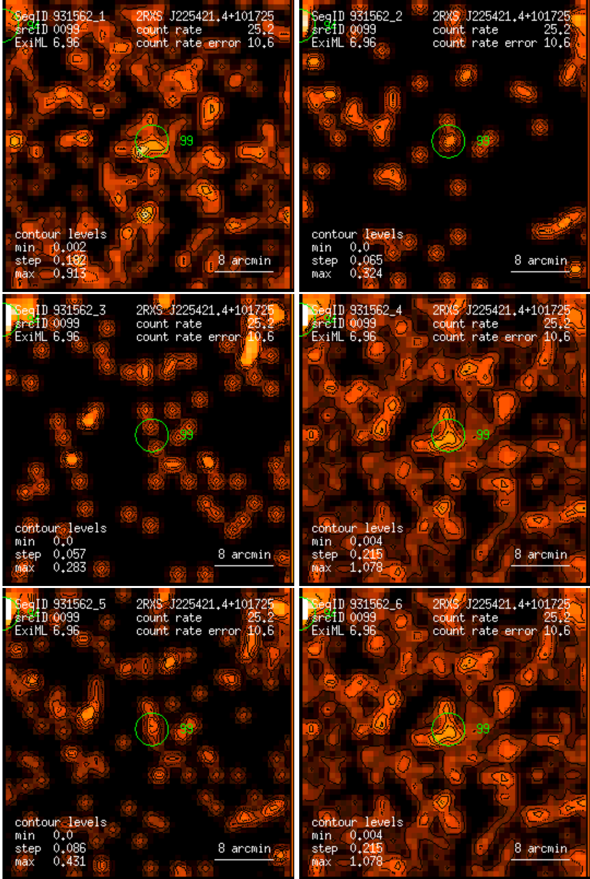
Figure 99: RASS 931562: detection 0099: band rate images, Gaussian filter: (1) PSPC channels 11 – 41, (2) 52 – 90, (3) 91 – 201, (4) 11 – 235, (5) 52 – 201, (6) 11 – 201. Broad band rates in counts/ks. Band rate contour levels in counts/ks/arcmin 2 .
