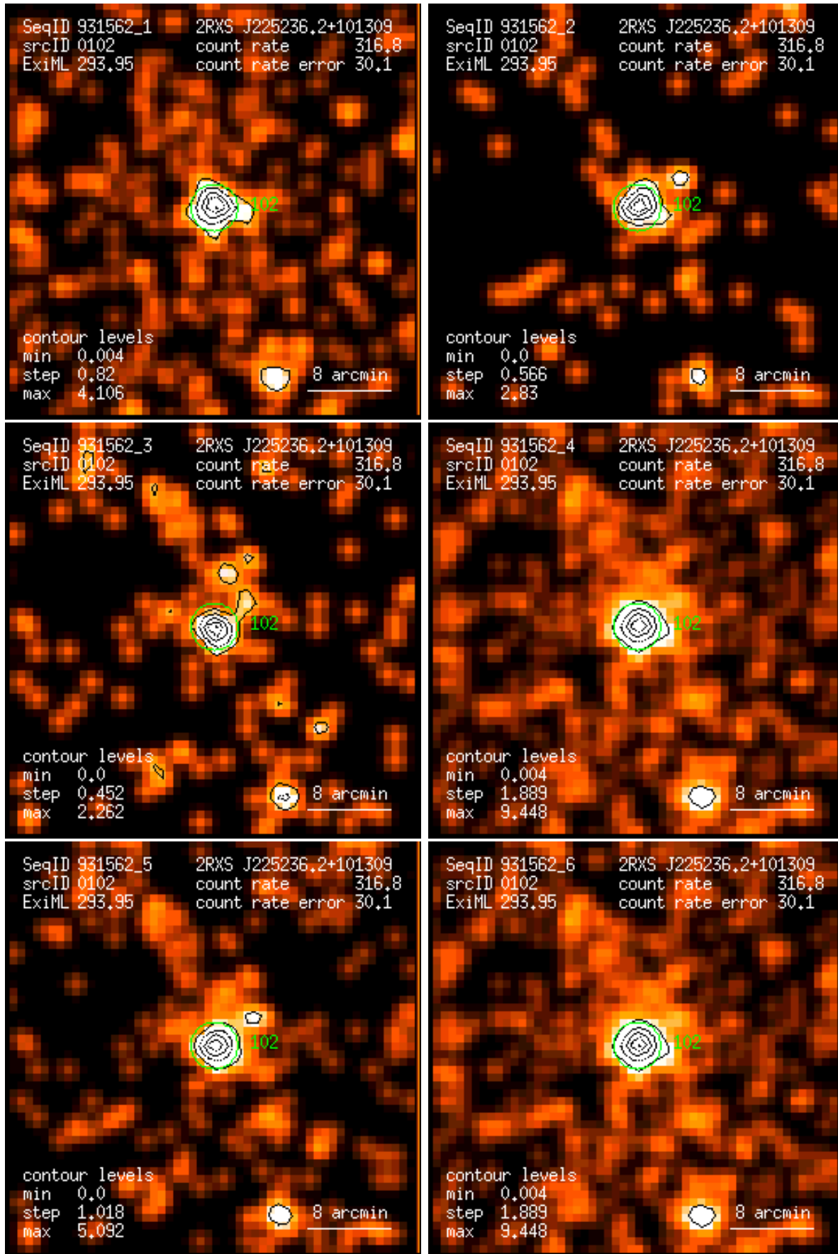
Figure 102: RASS 931562: detection 0102: band rate images, Gaussian filter: (1) PSPC channels 11 – 41, (2) 52 – 90, (3) 91 – 201, (4) 11 – 235, (5) 52 – 201, (6) 11 – 201. Broad band rates in counts/ks. Band rate contour levels in counts/ks/arcmin 2 .
