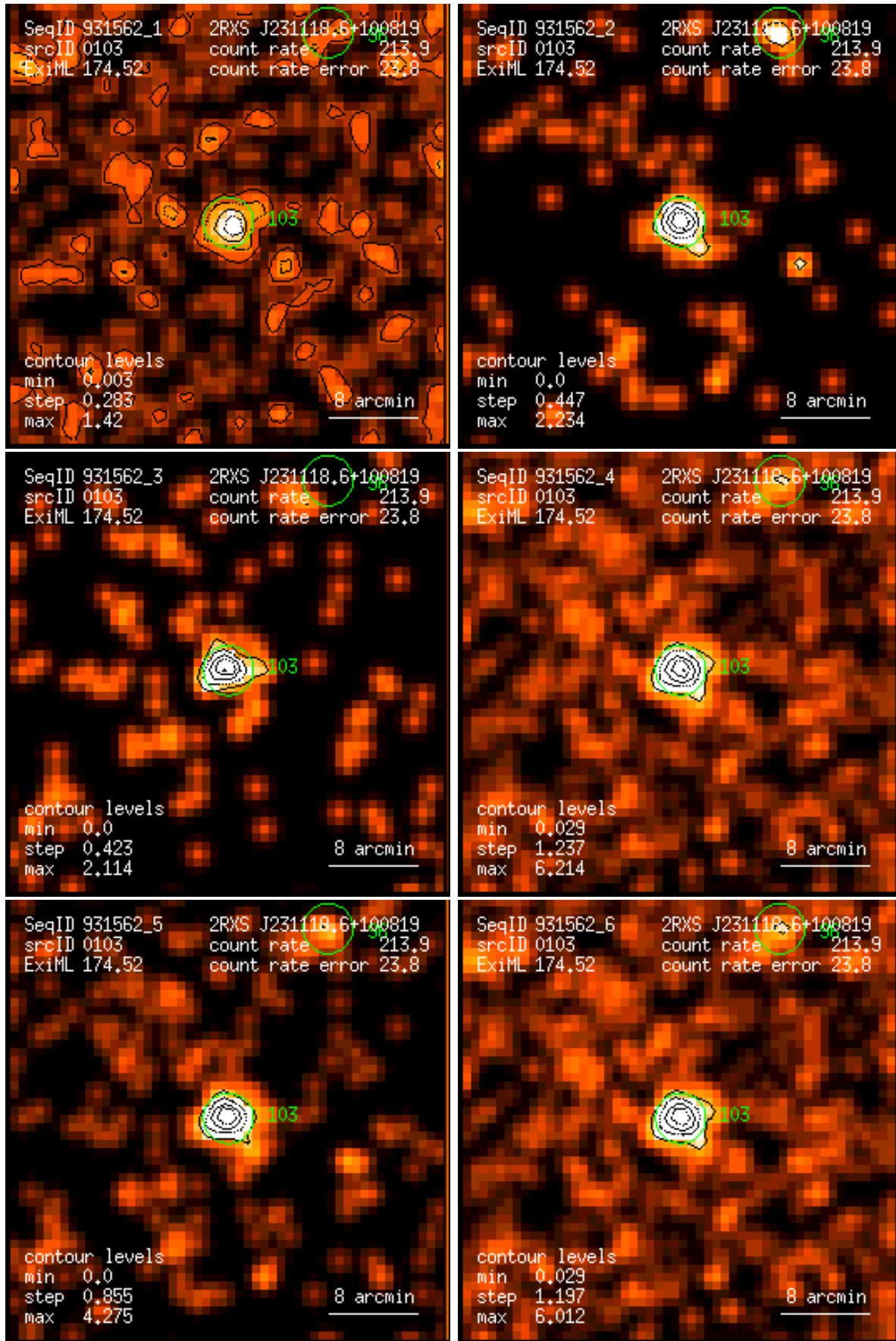
Figure 103: RASS 931562: detection 0103: band rate images, Gaussian filter: (1) PSPC channels 11 – 41, (2) 52 – 90, (3) 91 – 201, (4) 11 – 235, (5) 52 – 201, (6) 11 – 201. Broad band rates in counts/ks. Band rate contour levels in counts/ks/arcmin 2 .
