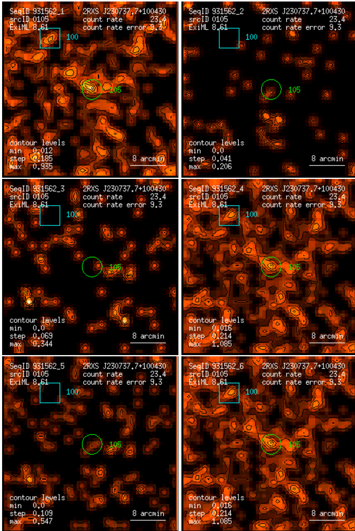
Figure 105: RASS 931562: detection 0105: band rate images, Gaussian filter: (1) PSPC channels 11 – 41, (2) 52 – 90, (3) 91 – 201, (4) 11 – 235, (5) 52 – 201, (6) 11 – 201. Broad band rates in counts/ks. Band rate contour levels in counts/ks/arcmin 2 .
