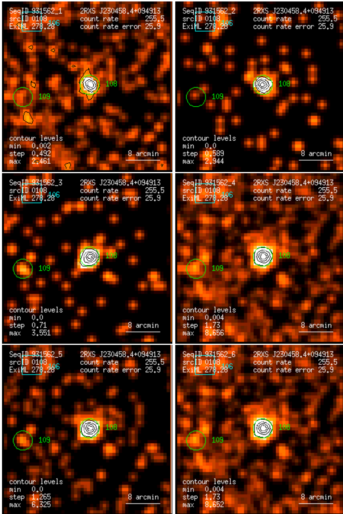
Figure 108: RASS 931562: detection 0108: band rate images, Gaussian filter: (1) PSPC channels 11 – 41, (2) 52 – 90, (3) 91 – 201, (4) 11 – 235, (5) 52 – 201, (6) 11 – 201. Broad band rates in counts/ks. Band rate contour levels in counts/ks/arcmin 2 .
