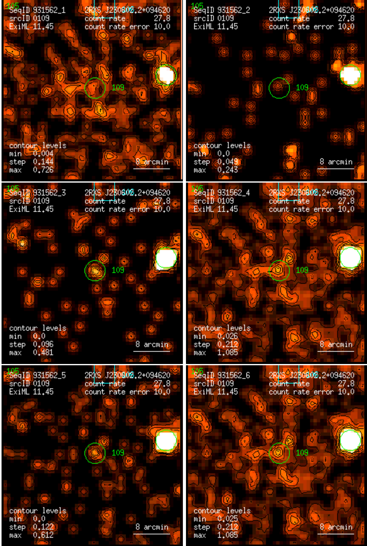
Figure 109: RASS 931562: detection 0109: band rate images, Gaussian filter: (1) PSPC channels 11 – 41, (2) 52 – 90, (3) 91 – 201, (4) 11 – 235, (5) 52 – 201, (6) 11 – 201. Broad band rates in counts/ks. Band rate contour levels in counts/ks/arcmin 2 .
