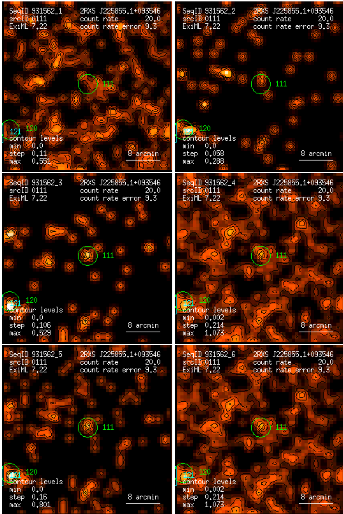
Figure 111: RASS 931562: detection 0111: band rate images, Gaussian filter: (1) PSPC channels 11 – 41, (2) 52 – 90, (3) 91 – 201, (4) 11 – 235, (5) 52 – 201, (6) 11 – 201. Broad band rates in counts/ks. Band rate contour levels in counts/ks/arcmin 2 .
