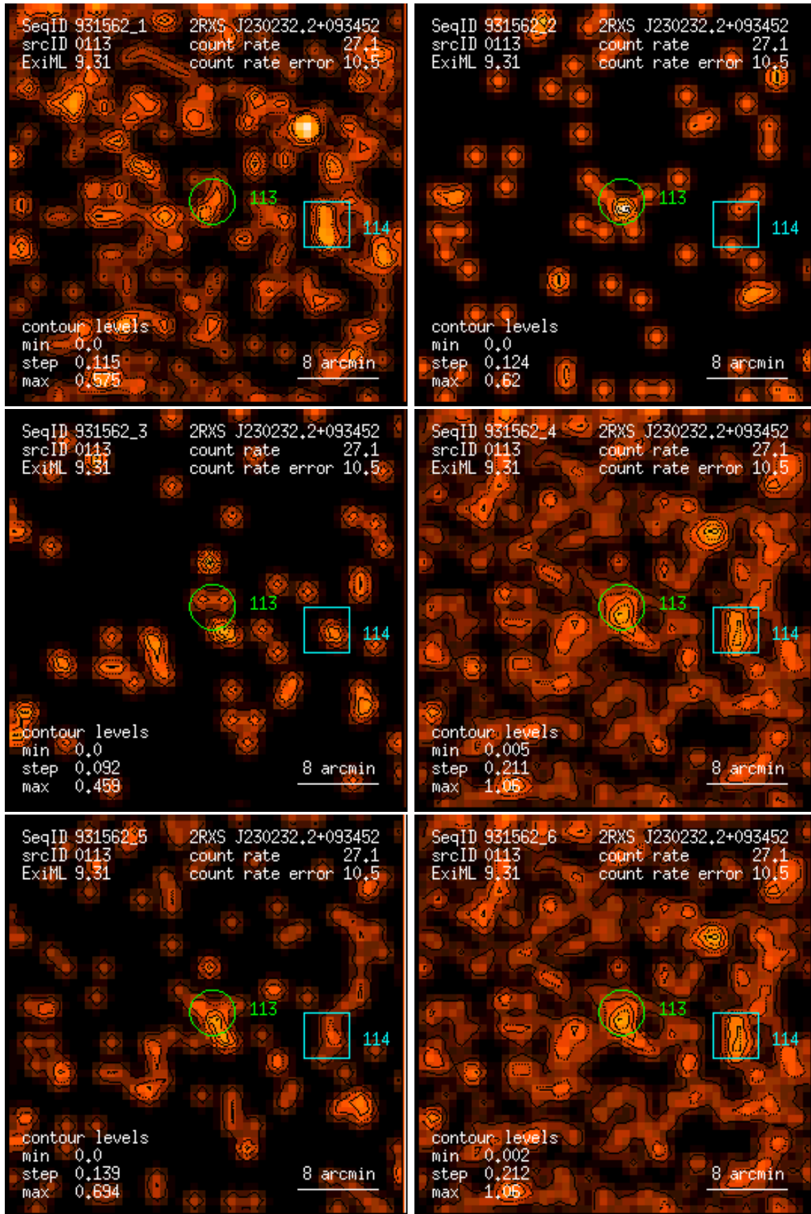
Figure 113: RASS 931562: detection 0113: band rate images, Gaussian filter: (1) PSPC channels 11 – 41, (2) 52 – 90, (3) 91 – 201, (4) 11 – 235, (5) 52 – 201, (6) 11 – 201. Broad band rates in counts/ks. Band rate contour levels in counts/ks/arcmin 2 .
