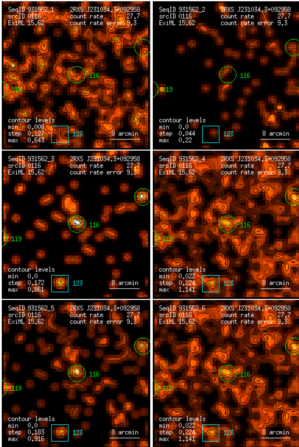
Figure 116: RASS 931562: detection 0116: band rate images, Gaussian filter: (1) PSPC channels 11 – 41, (2) 52 – 90, (3) 91 – 201, (4) 11 – 235, (5) 52 – 201, (6) 11 – 201. Broad band rates in counts/ks. Band rate contour levels in counts/ks/arcmin 2 .
