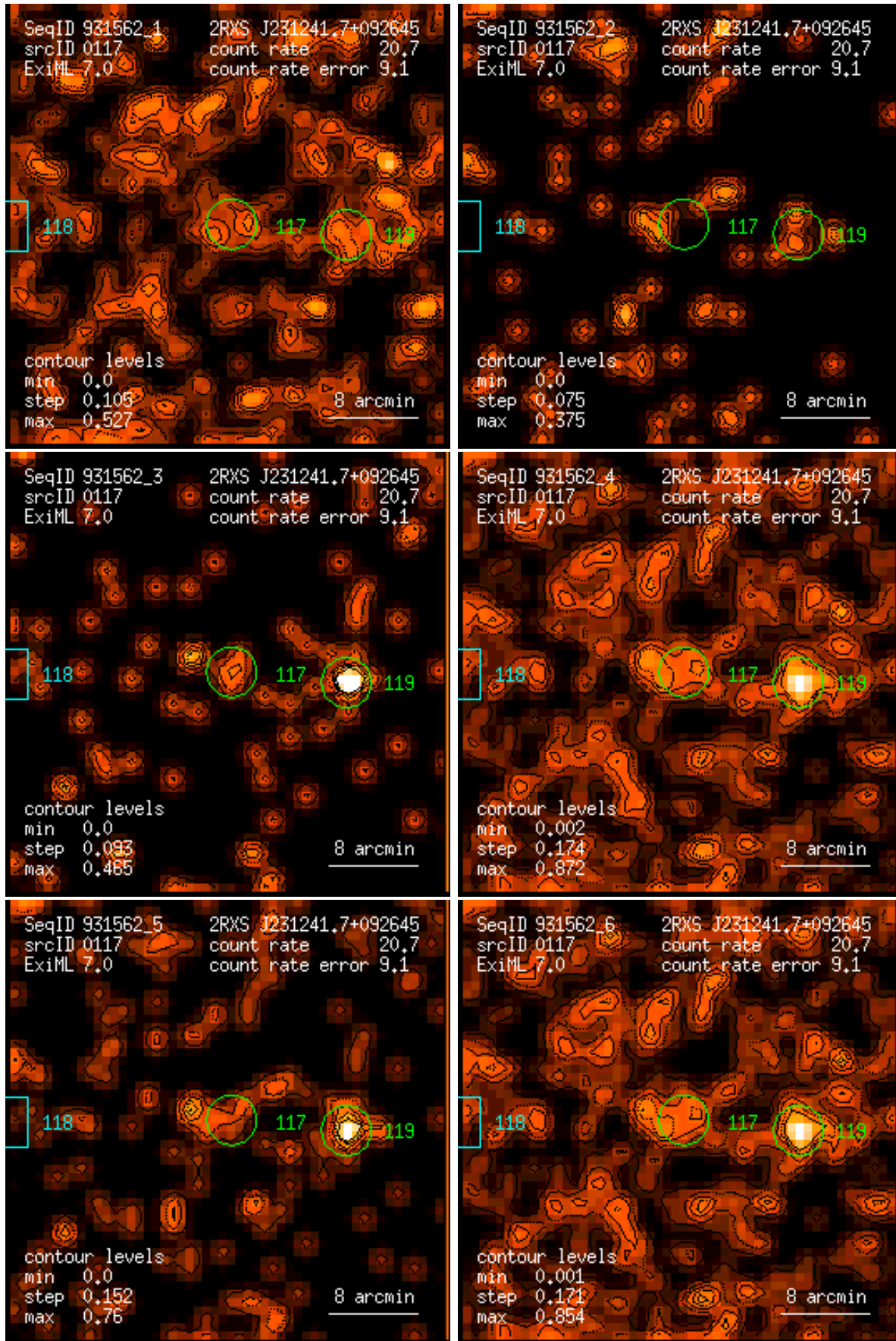
Figure 117: RASS 931562: detection 0117: band rate images, Gaussian filter: (1) PSPC channels 11 – 41, (2) 52 – 90, (3) 91 – 201, (4) 11 – 235, (5) 52 – 201, (6) 11 – 201. Broad band rates in counts/ks. Band rate contour levels in counts/ks/arcmin 2 .
