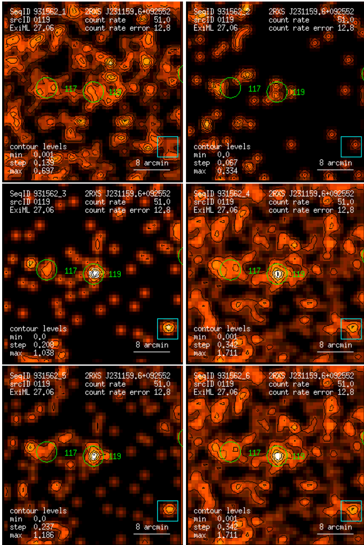
Figure 119: RASS 931562: detection 0119: band rate images, Gaussian filter: (1) PSPC channels 11 – 41, (2) 52 – 90, (3) 91 – 201, (4) 11 – 235, (5) 52 – 201, (6) 11 – 201. Broad band rates in counts/ks. Band rate contour levels in counts/ks/arcmin 2 .
