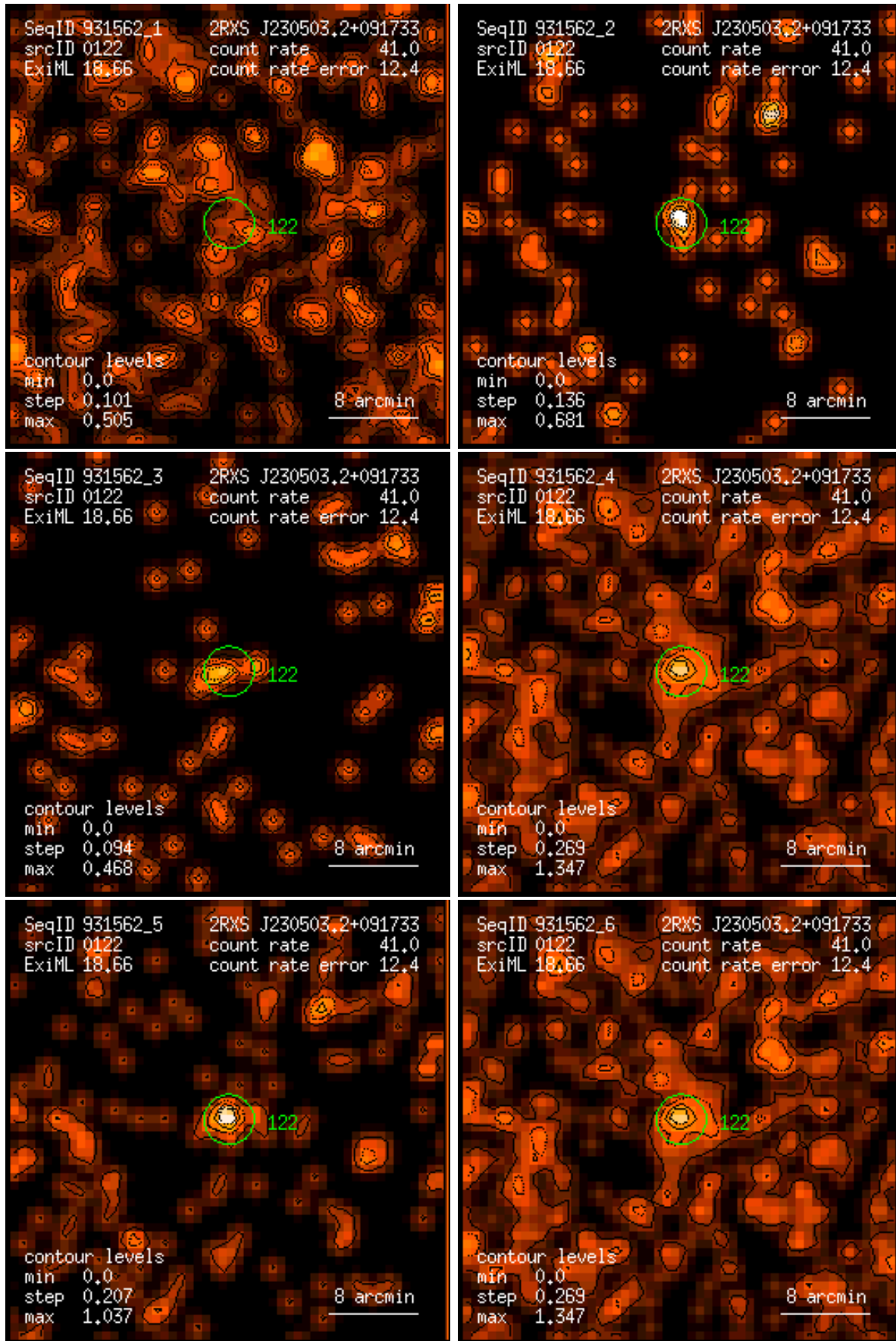
Figure 122: RASS 931562: detection 0122: band rate images, Gaussian filter: (1) PSPC channels 11 – 41, (2) 52 – 90, (3) 91 – 201, (4) 11 – 235, (5) 52 – 201, (6) 11 – 201. Broad band rates in counts/ks. Band rate contour levels in counts/ks/arcmin 2 .
