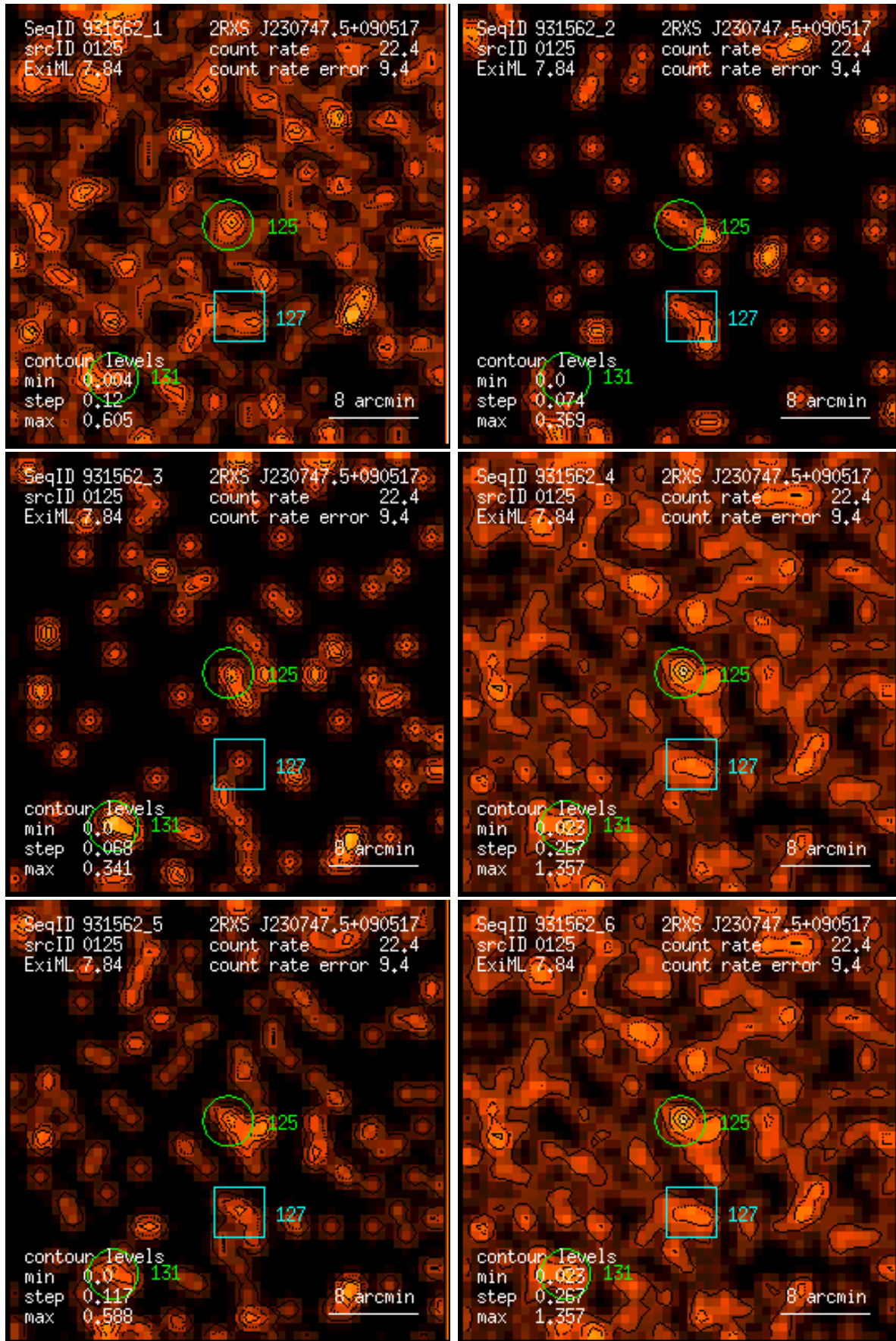
Figure 125: RASS 931562: detection 0125: band rate images, Gaussian filter: (1) PSPC channels 11 – 41, (2) 52 – 90, (3) 91 – 201, (4) 11 – 235, (5) 52 – 201, (6) 11 – 201. Broad band rates in counts/ks. Band rate contour levels in counts/ks/arcmin 2 .
