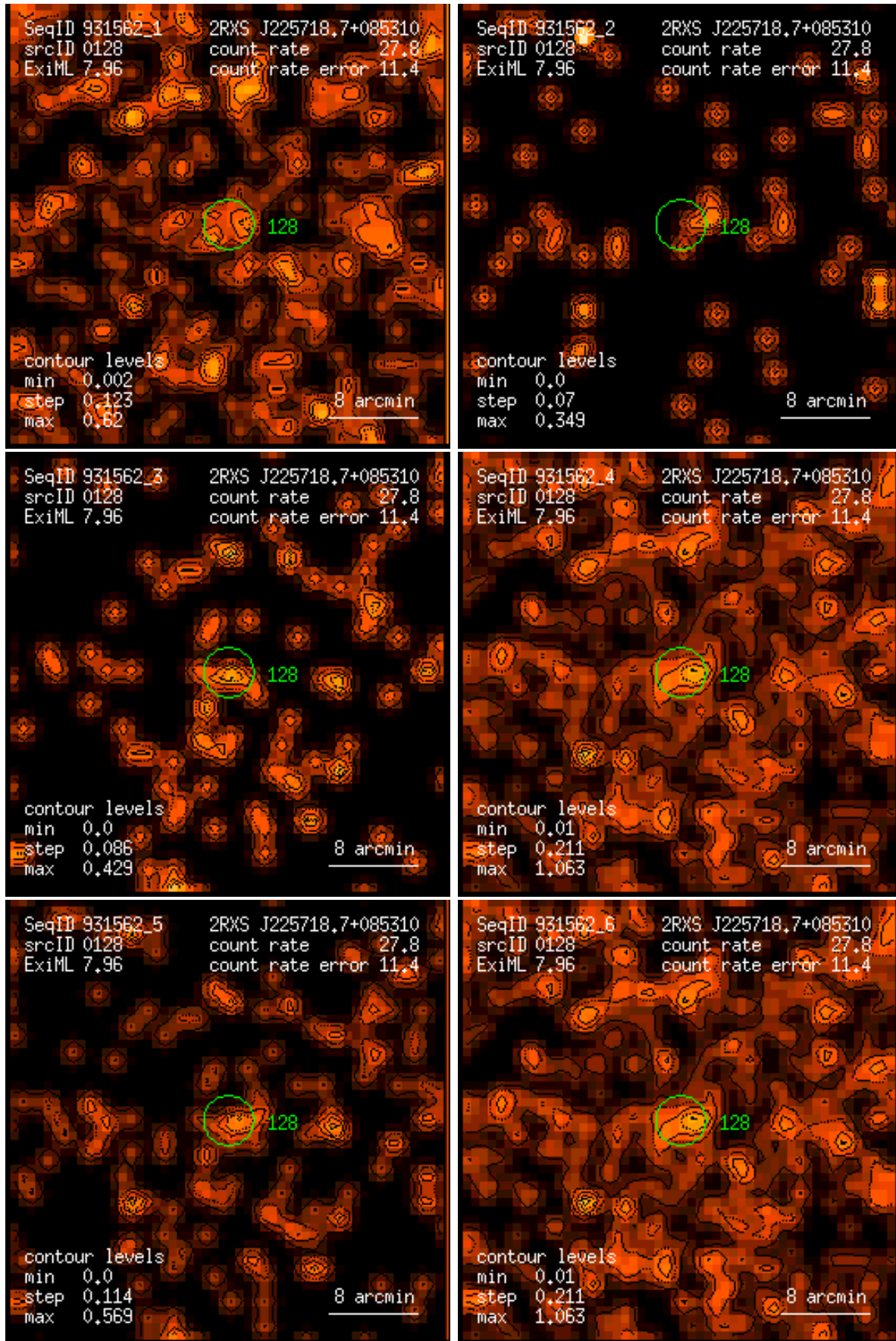
Figure 128: RASS 931562: detection 0128: band rate images, Gaussian filter: (1) PSPC channels 11 – 41, (2) 52 – 90, (3) 91 – 201, (4) 11 – 235, (5) 52 – 201, (6) 11 – 201. Broad band rates in counts/ks. Band rate contour levels in counts/ks/arcmin 2 .
