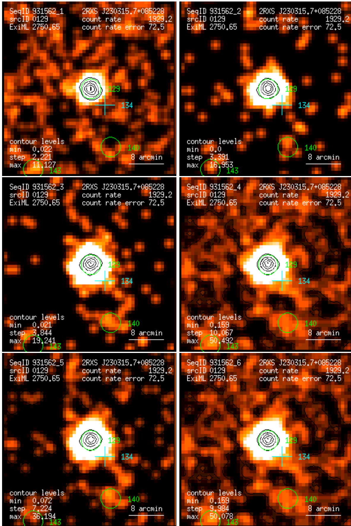
Figure 129: RASS 931562: detection 0129: band rate images, Gaussian filter: (1) PSPC channels 11 – 41, (2) 52 – 90, (3) 91 – 201, (4) 11 – 235, (5) 52 – 201, (6) 11 – 201. Broad band rates in counts/ks. Band rate contour levels in counts/ks/arcmin 2 .
