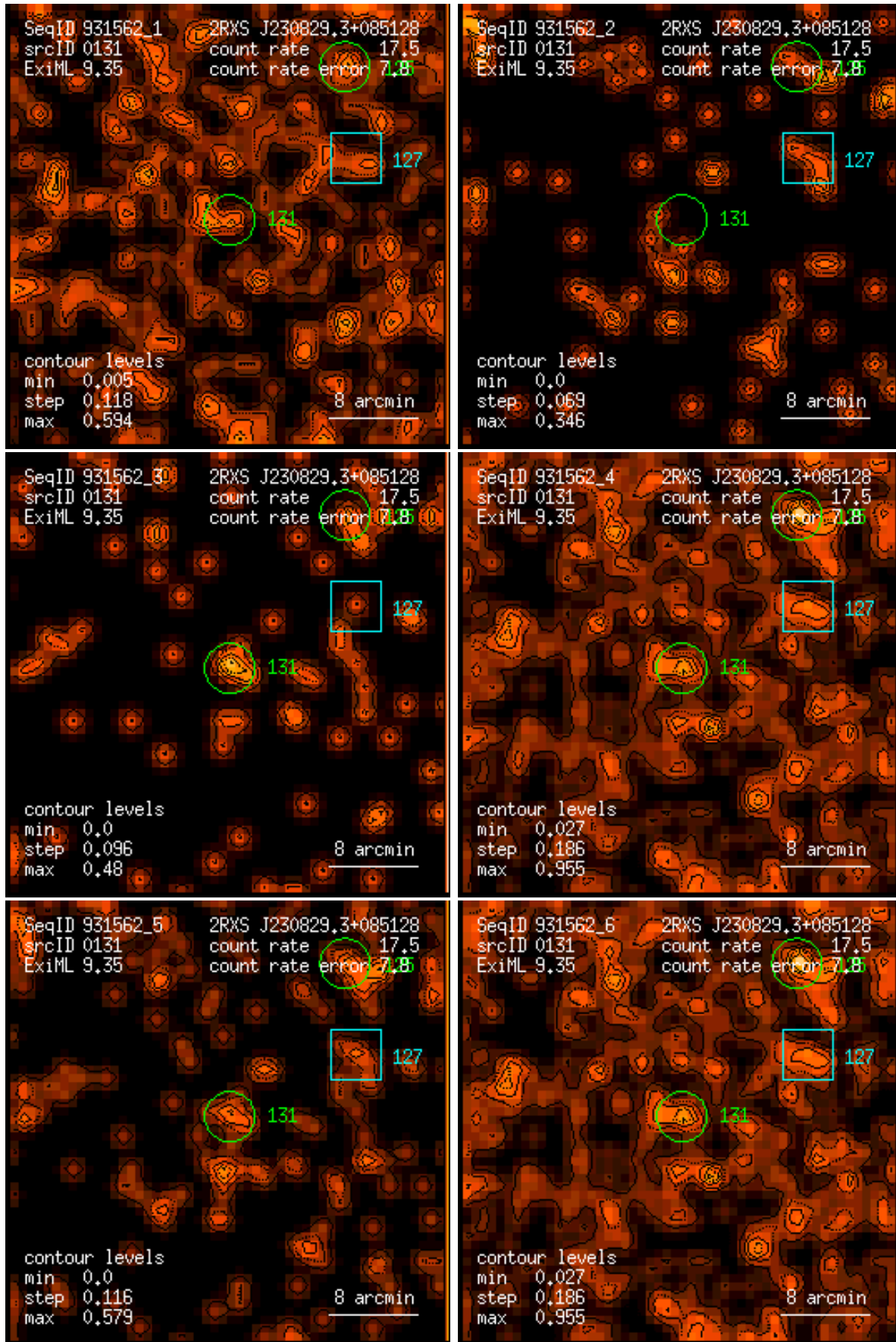
Figure 131: RASS 931562: detection 0131: band rate images, Gaussian filter: (1) PSPC channels 11 – 41, (2) 52 – 90, (3) 91 – 201, (4) 11 – 235, (5) 52 – 201, (6) 11 – 201. Broad band rates in counts/ks. Band rate contour levels in counts/ks/arcmin 2 .
